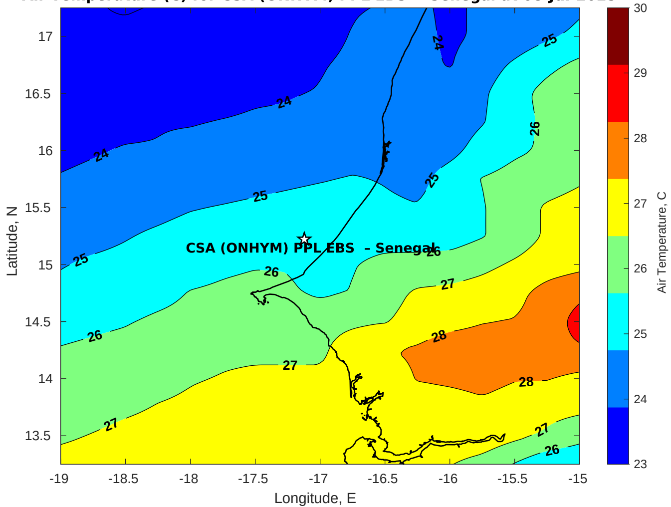
Air Temperature (C) for CSA (ONHYM) PPL EBS - Senegal at 08-Jul-2025
