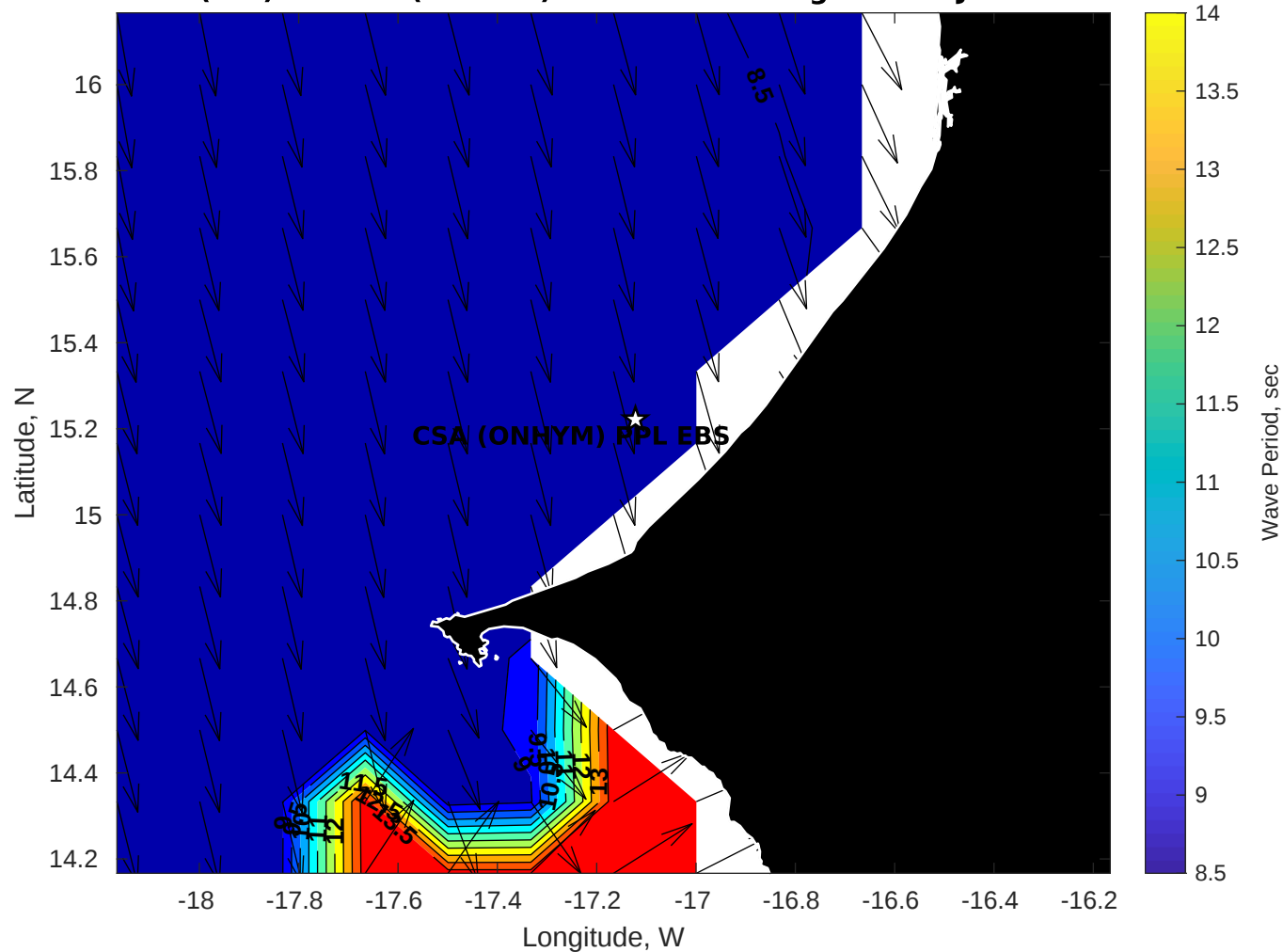
Wave Period (sec) for CSA (ONHYM) PPL EBS - Senegal at 08-Jul-2025 09:00:00
