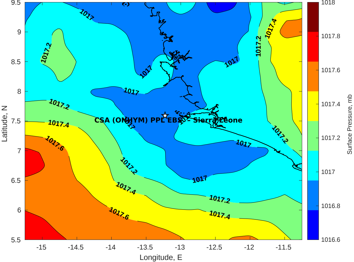
Surface Pressure (mb) for CSA (ONHYM) PPL EBS - Sierra Leone at 09-Jul-2025 00:00:00
