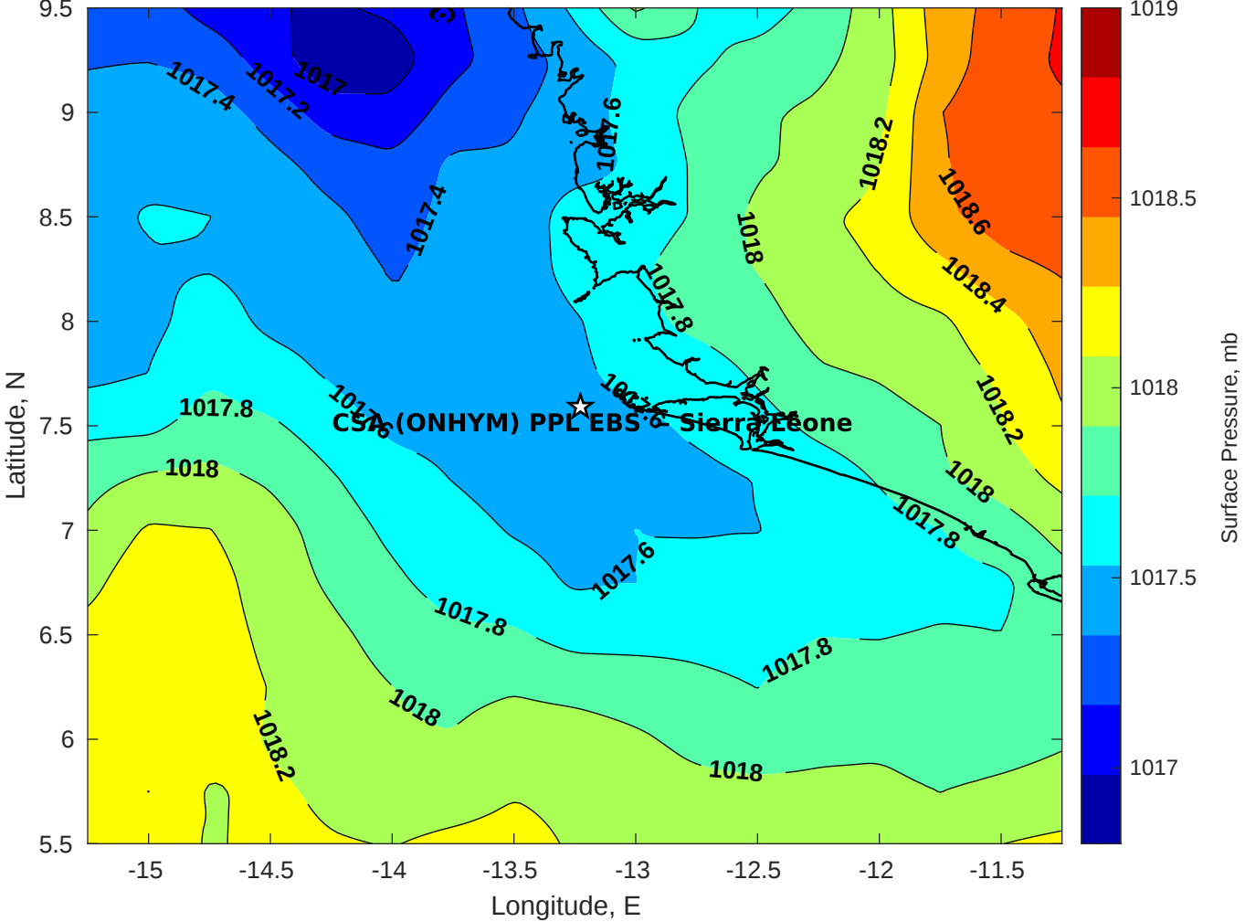
Surface Pressure (mb) for CSA (ONHYM) PPL EBS - Sierra Leone at 10-Jul-2025 00:00:00
