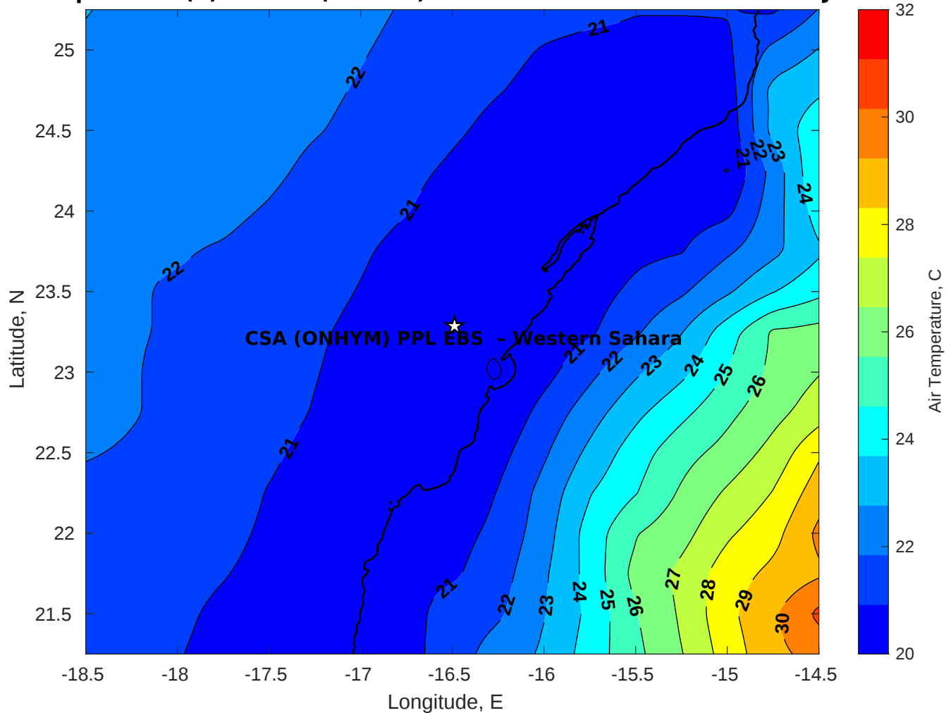
Air Temperature (C) for CSA (ONHYM) PPL EBS - Western Sahara at 08-Jul-2025
