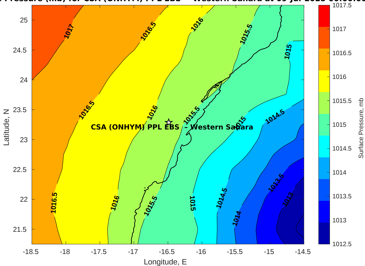
Surface Pressure (mb) for CSA (ONHYM) PPL EBS - Western Sahara at 09-Jul-2025 00:00:00
