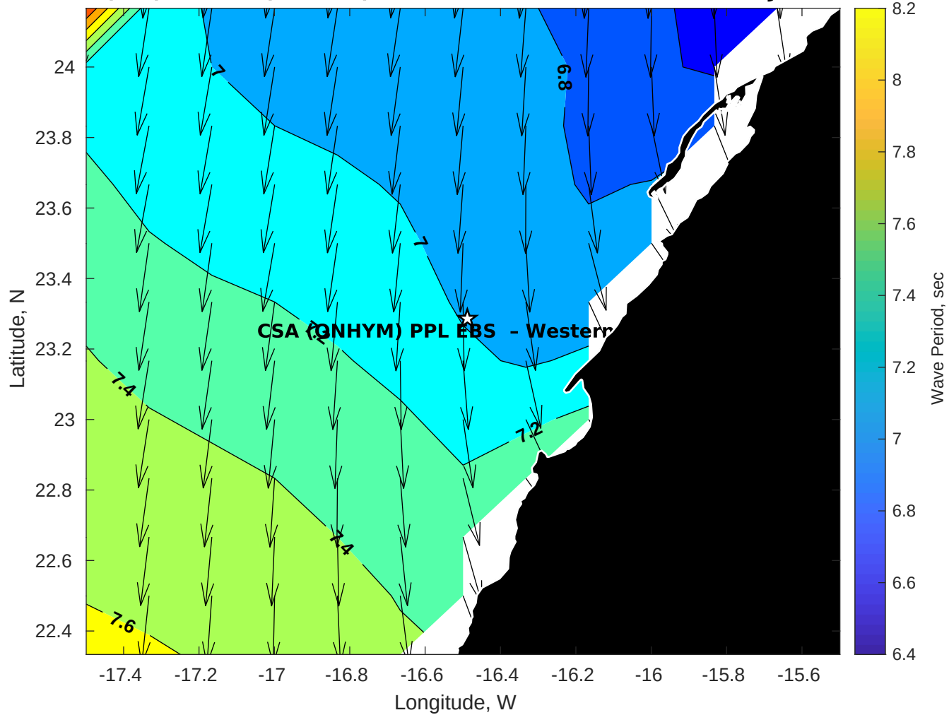
Wave Period (sec) for CSA (ONHYM) PPL EBS - Western Sahara at 08-Jul-2025 09:00:00
