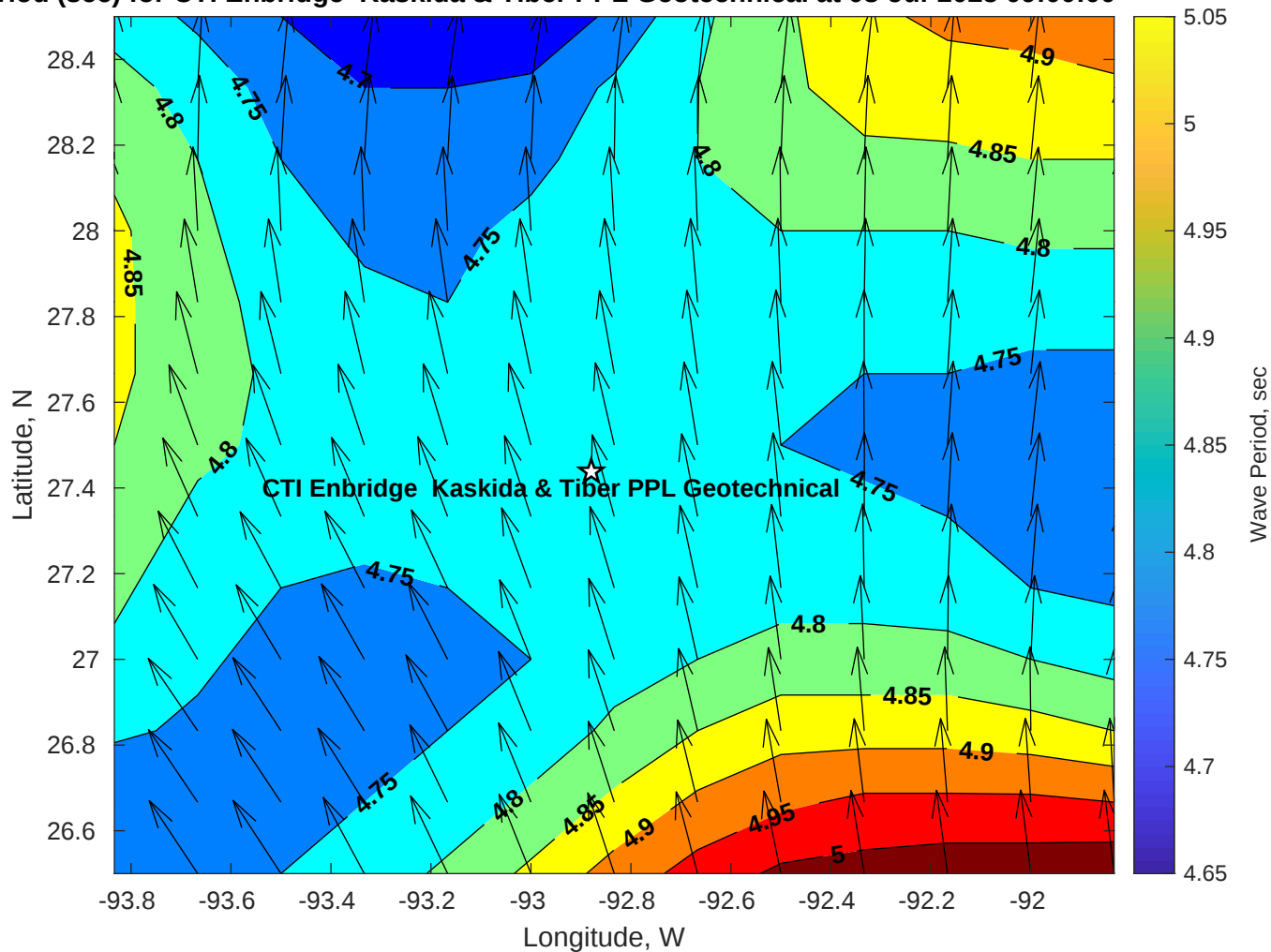
Wave Period (sec) for CTI Enbridge Kaskida & Tiber PPL Geotechnical at 08-Jul-2025 09:00:00
