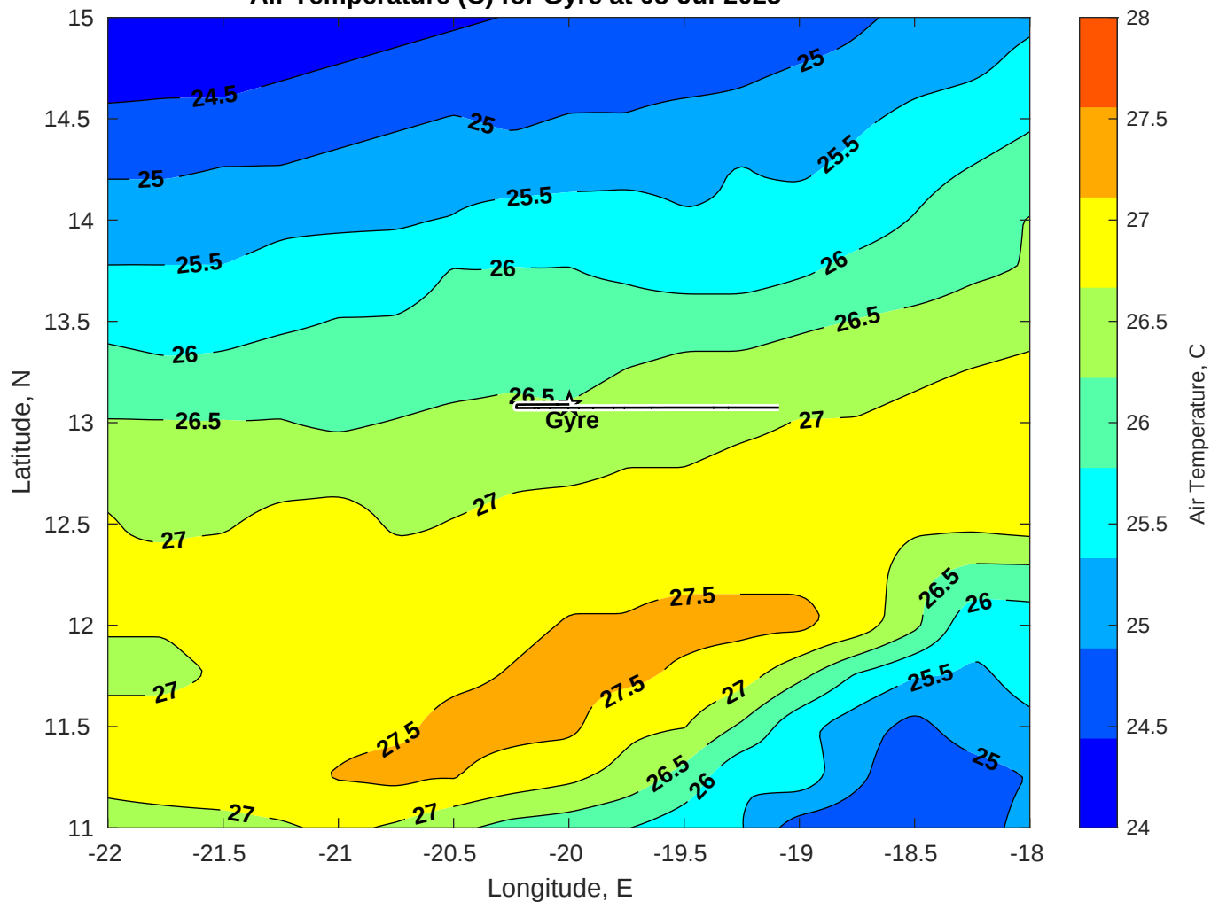
Air Temperature (C) for Gyre at 08-Jul-2025
