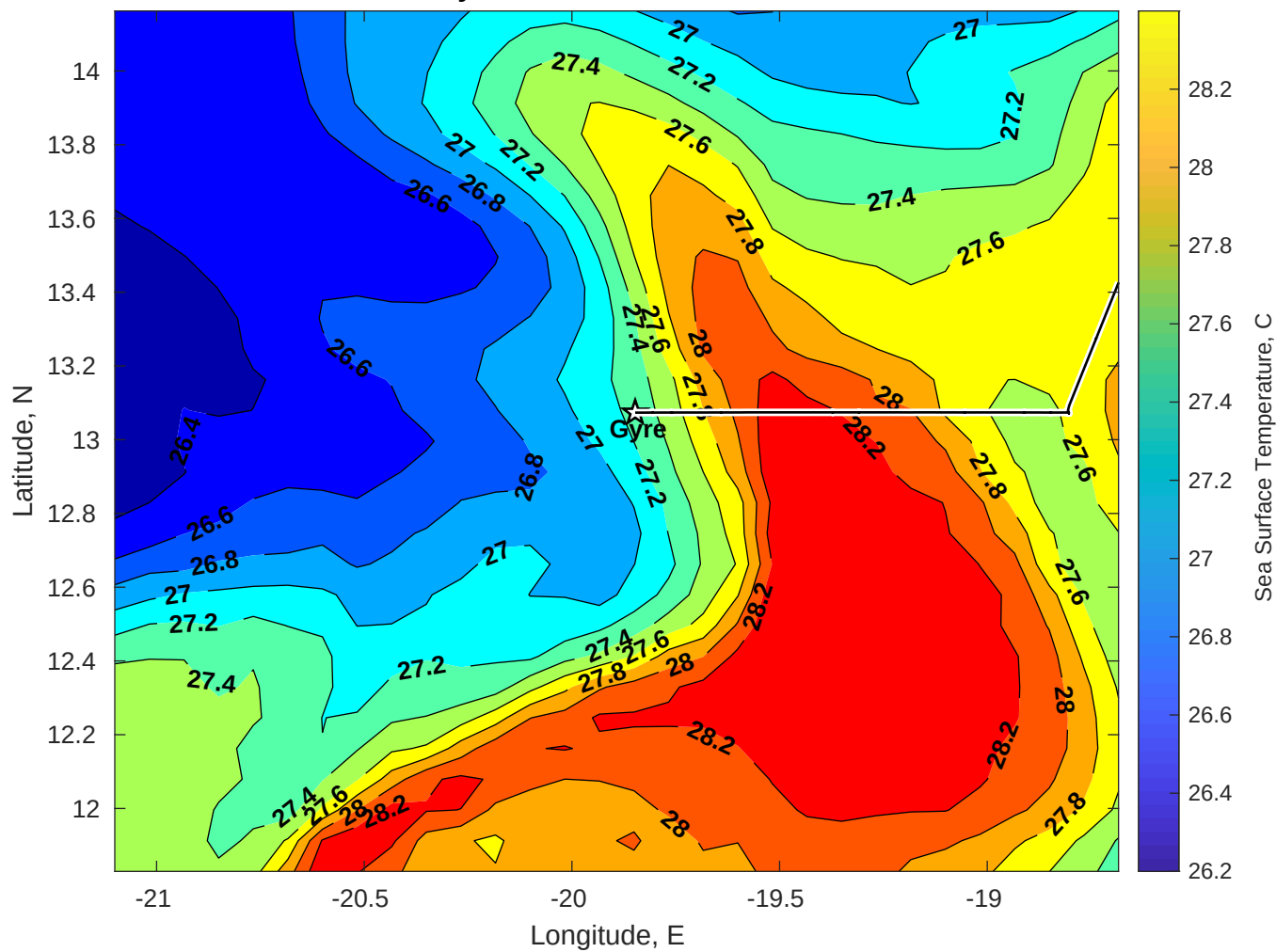
SST for Gyre at 07-Jul-2025 00:00:00
