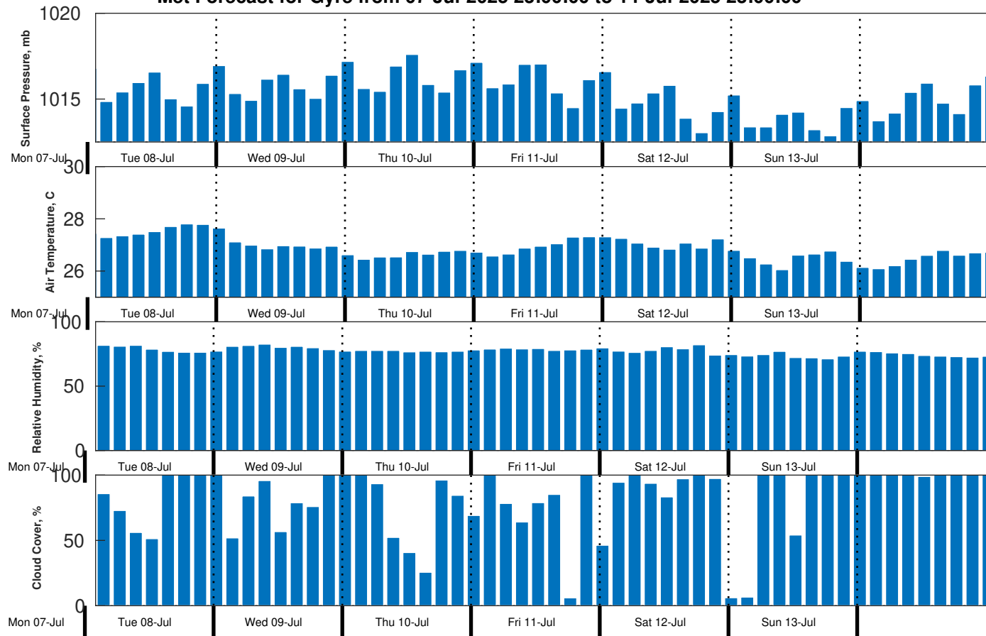
Met Forecast for Gyre from 07-Jul-2025 23:00:00 to 14-Jul-2025 23:00:00
