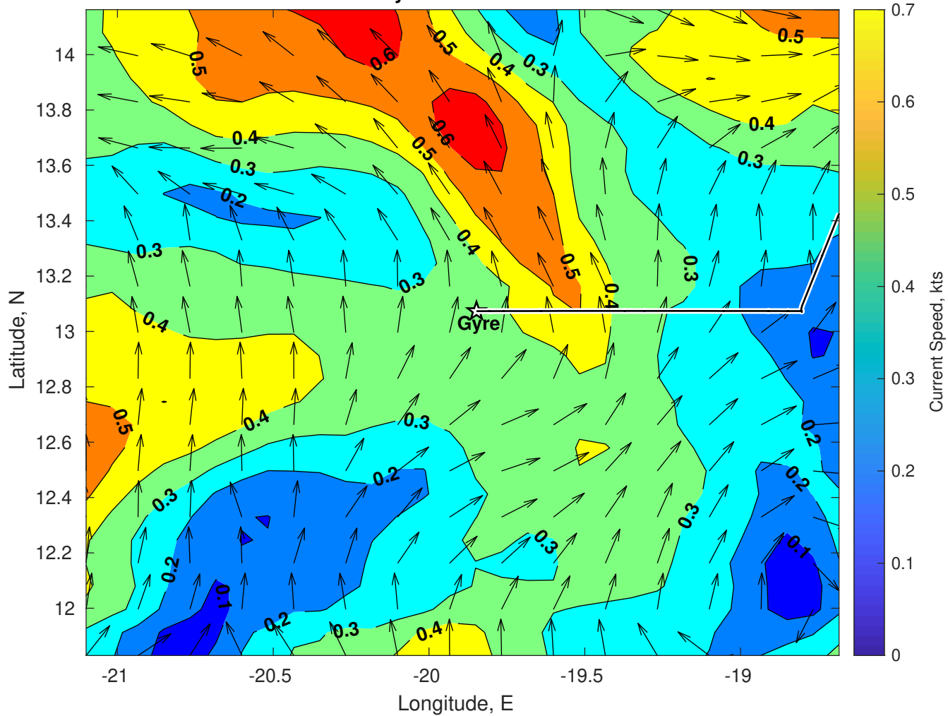
Surface Currents for Gyre at 07-Jul-2025 00:00:00
