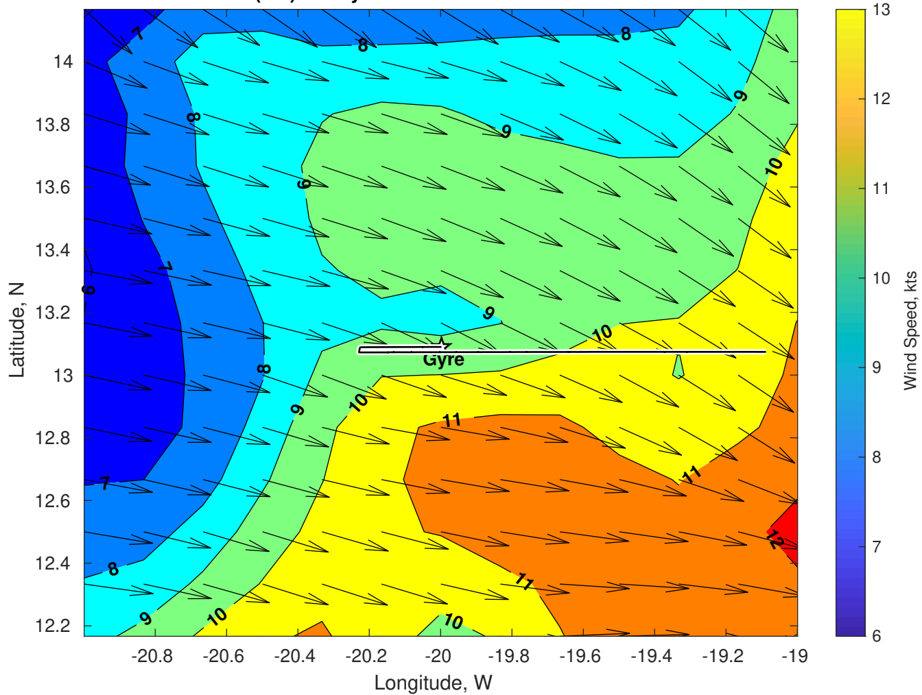
Winds (kts) for Gyre at 08-Jul-2025 09:00:00
