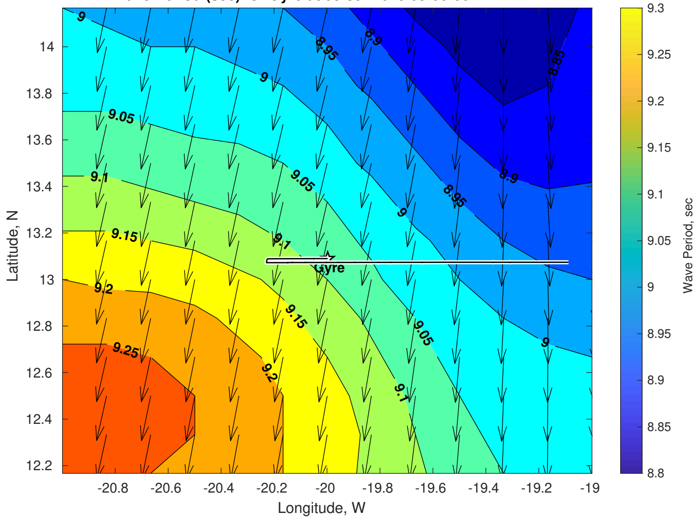
Wave Period (sec) for Gyre at 08-Jul-2025 09:00:00
