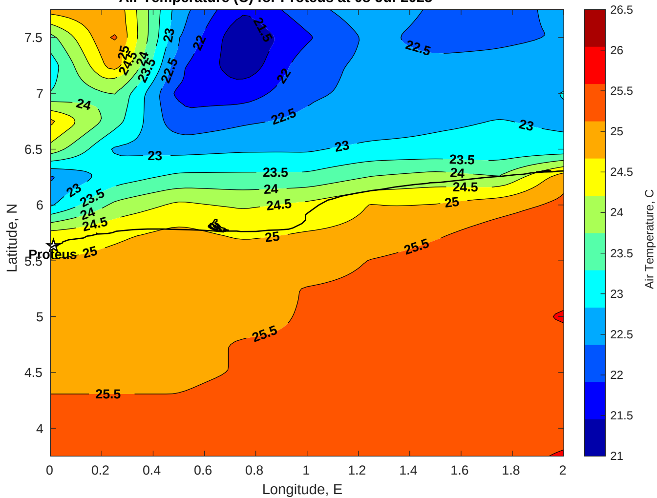
Air Temperature (C) for Proteus at 08-Jul-2025
