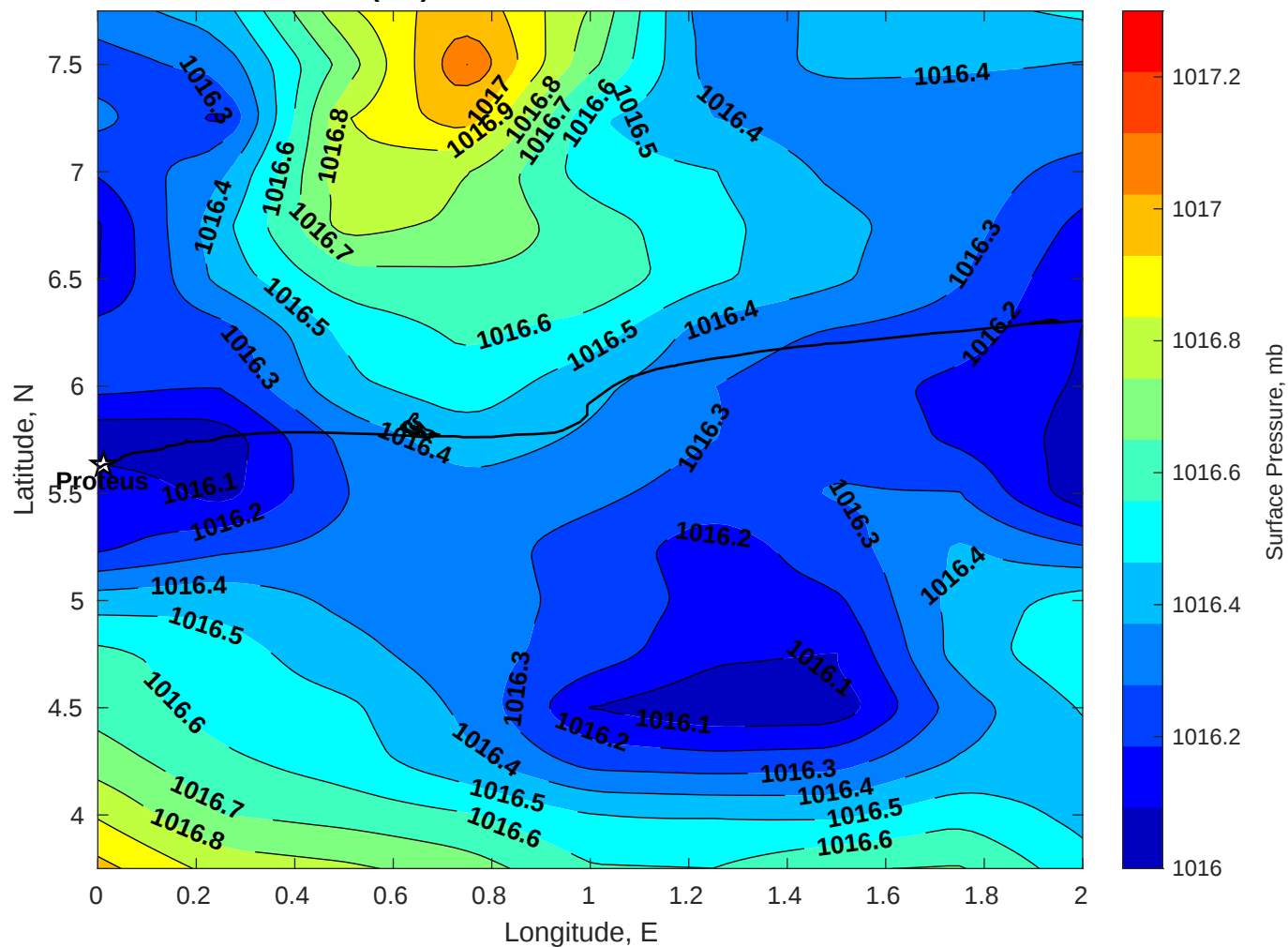
Surface Pressure (mb) for Proteus at 09-Jul-2025 00:00:00
