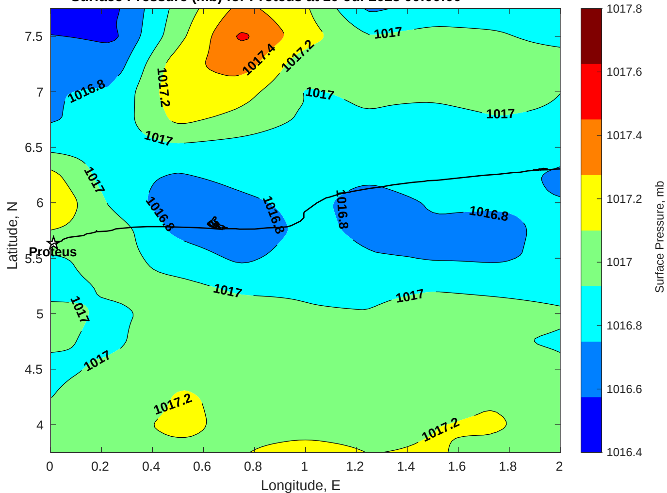
Surface Pressure (mb) for Proteus at 10-Jul-2025 00:00:00
