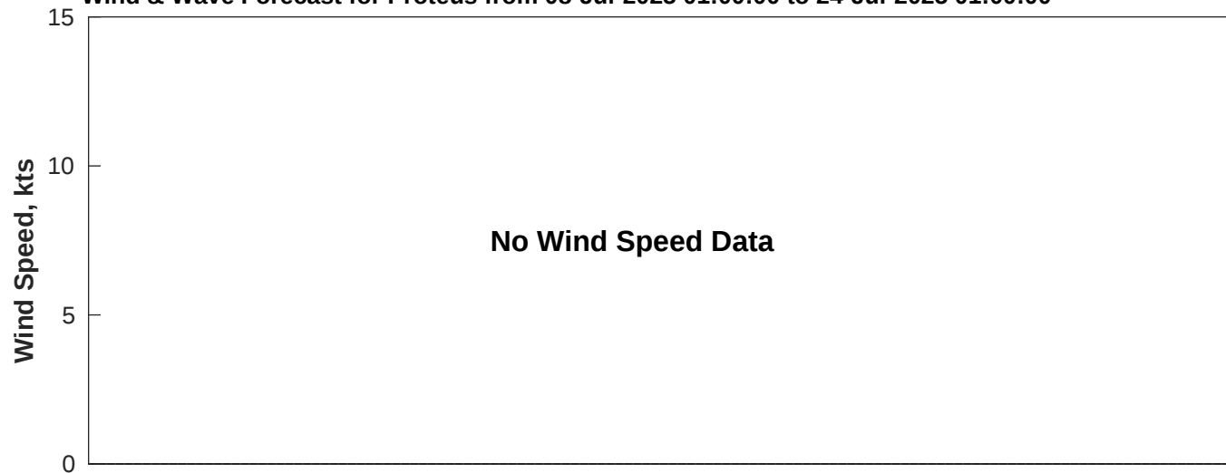
Wind & Wave Forecast for Proteus from 08-Jul-2025 01:00:00 to 24-Jul-2025 01:00:00
