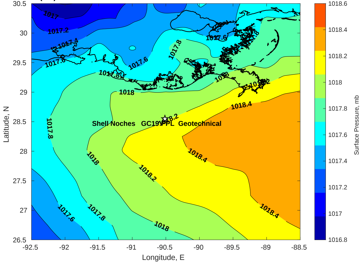
Surface Pressure (mb) for Shell Noches GC19 PPL Geotechnical at 08-Jul-2025 00:00:00
