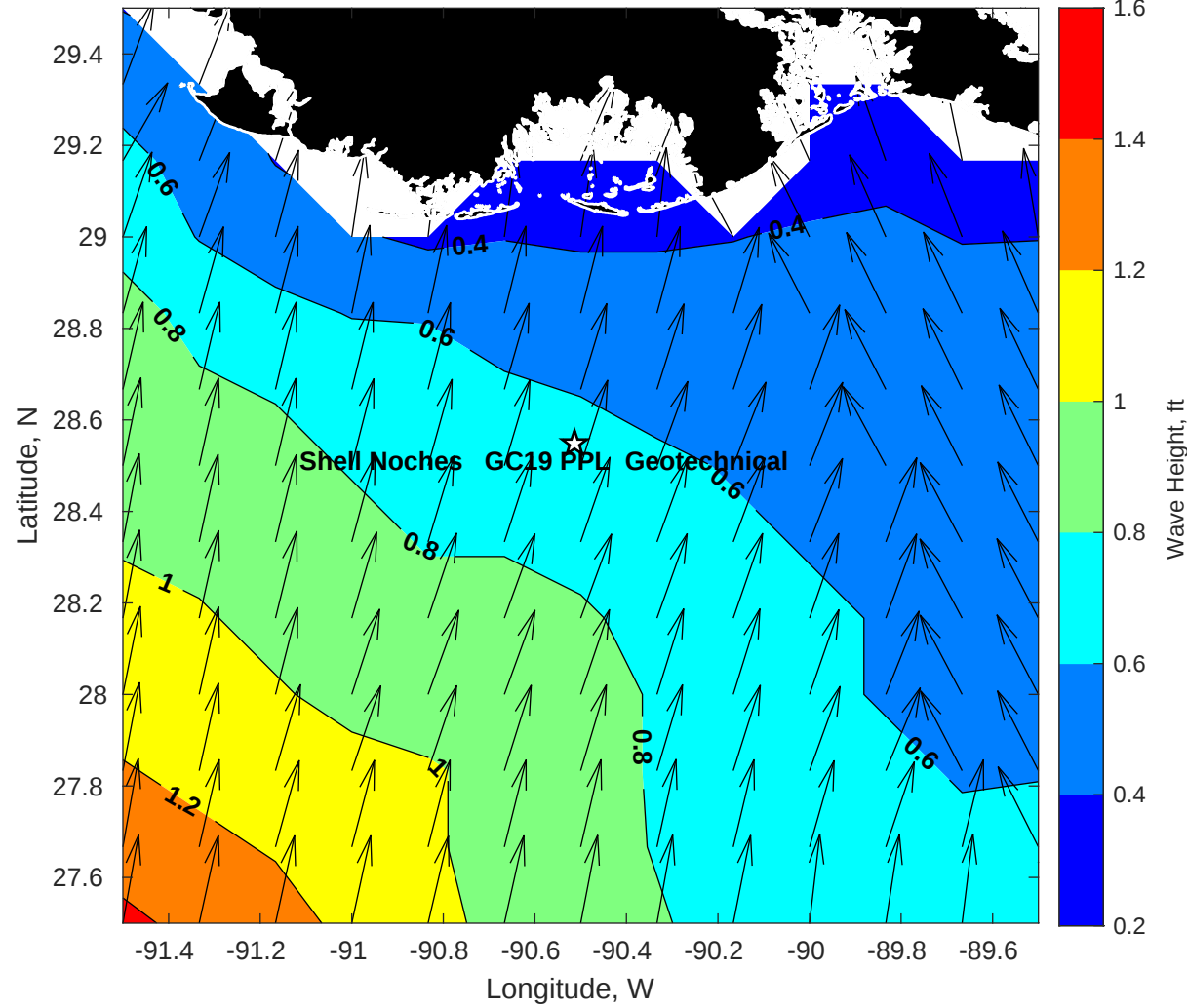
Wave Height (ft) for Shell Noches GC19 PPL Geotechnical at 08-Jul-2025 09:00:00
