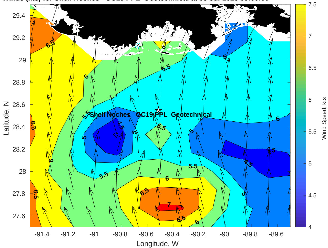
Winds (kts) for Shell Noches GC19 PPL Geotechnical at 08-Jul-2025 09:00:00
