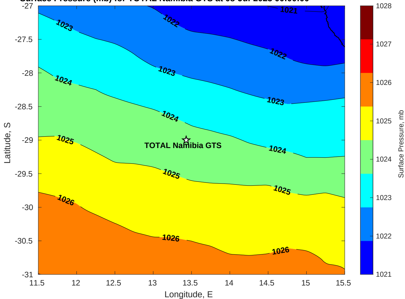
Surface Pressure (mb) for TOTAL Namibia GTS at 08-Jul-2025 00:00:00
