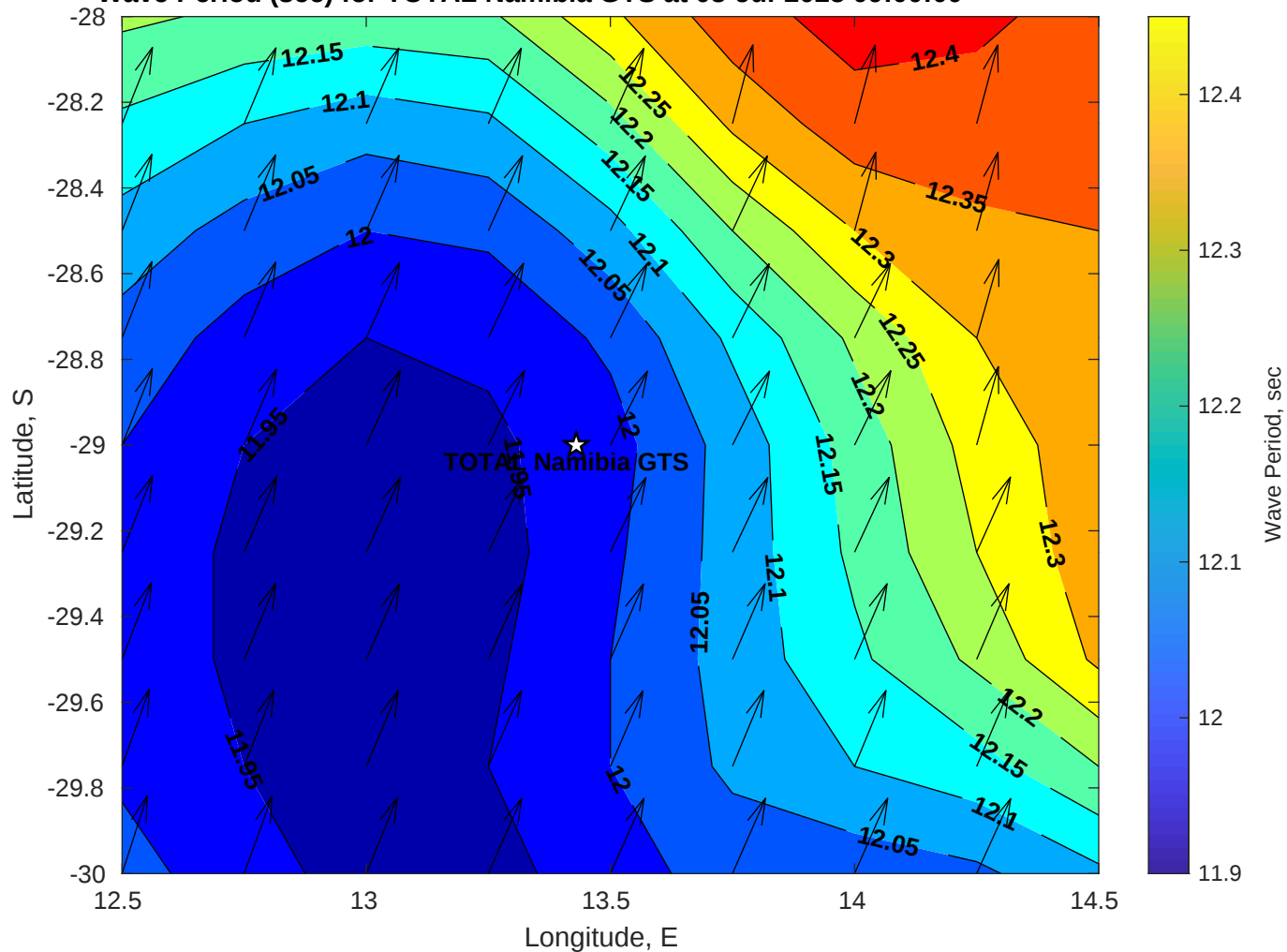
Wave Period (sec) for TOTAL Namibia GTS at 08-Jul-2025 09:00:00
