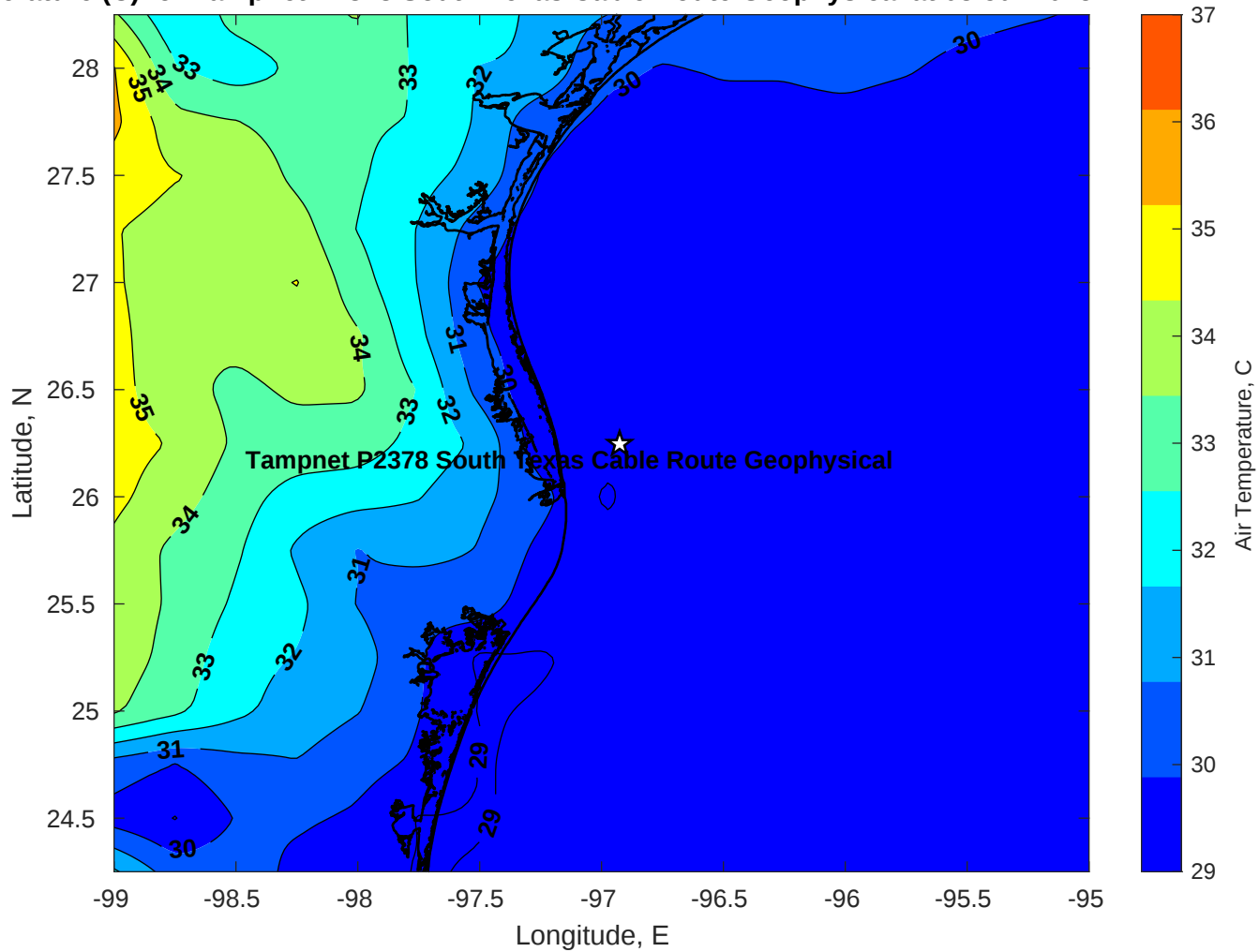
Air Temperature (C) for Tampnet P2378 South Texas Cable Route Geophysical at 08-Jul-2025
