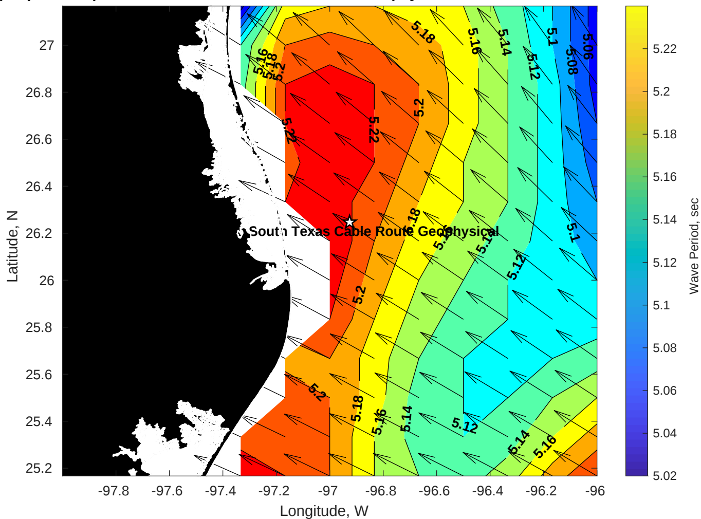
Wave Period (sec) for Tampnet P2378 South Texas Cable Route Geophysical at 08-Jul-2025 09:00:00
