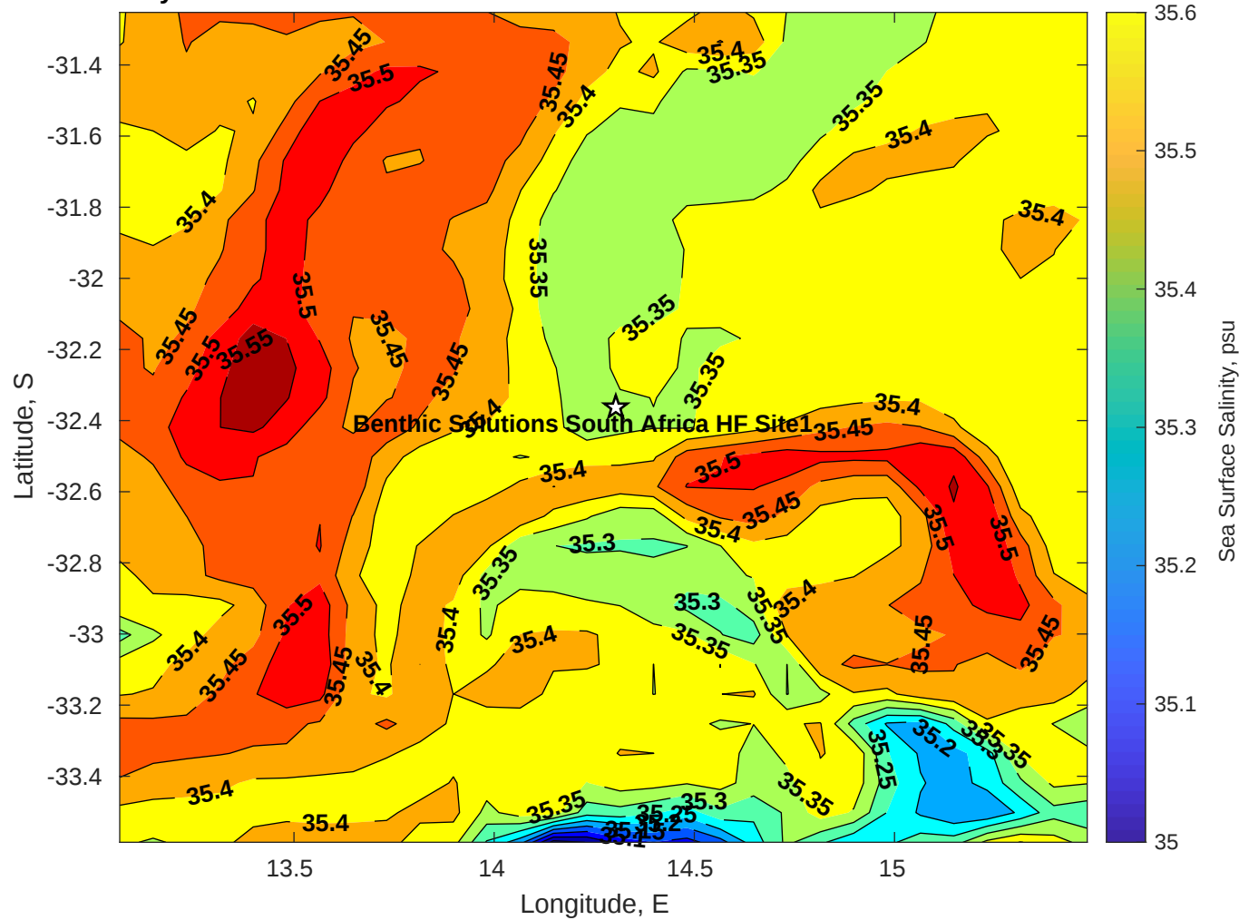
Surface Salinity for Benthic Solutions South Africa HF Site1 at 08-Jul-2025 00:00:00
