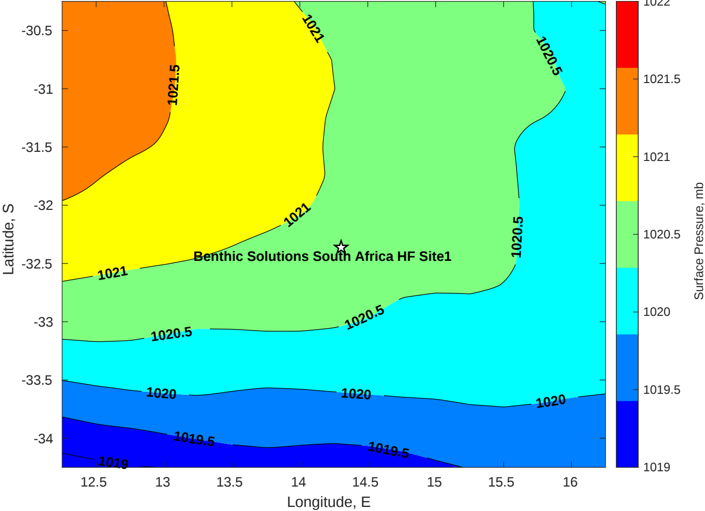
Surface Pressure (mb) for Benthic Solutions South Africa HF Site1 at 09-Jul-2025 00:00:00
