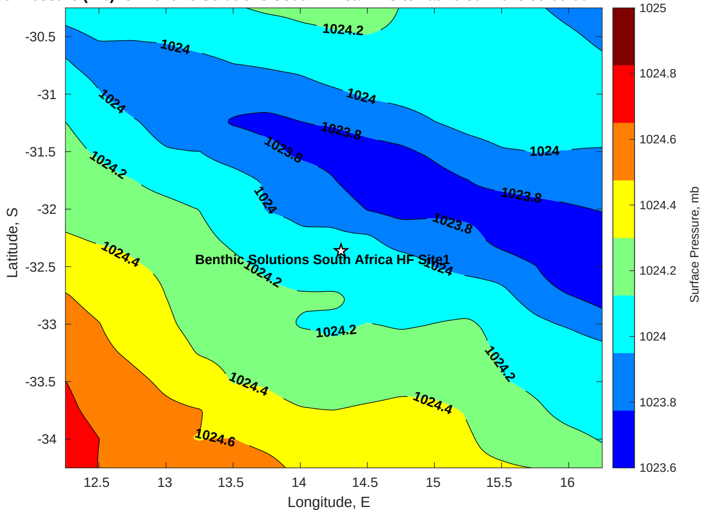
Surface Pressure (mb) for Benthic Solutions South Africa HF Site1 at 10-Jul-2025 00:00:00
