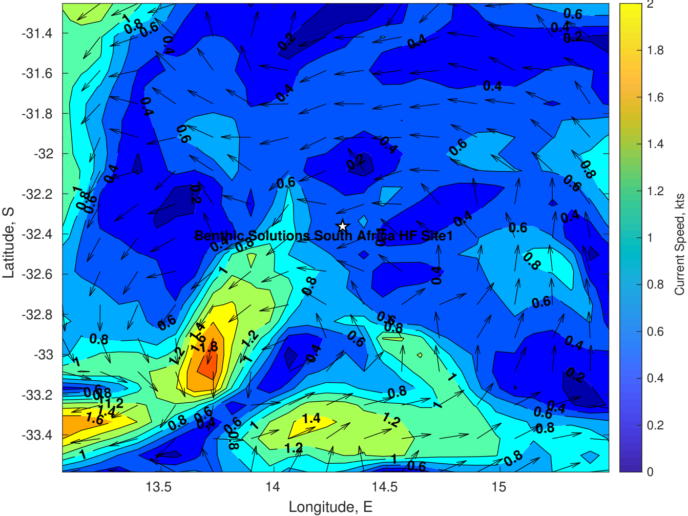
Surface Currents for Benthic Solutions South Africa HF Site1 at 08-Jul-2025 00:00:00
