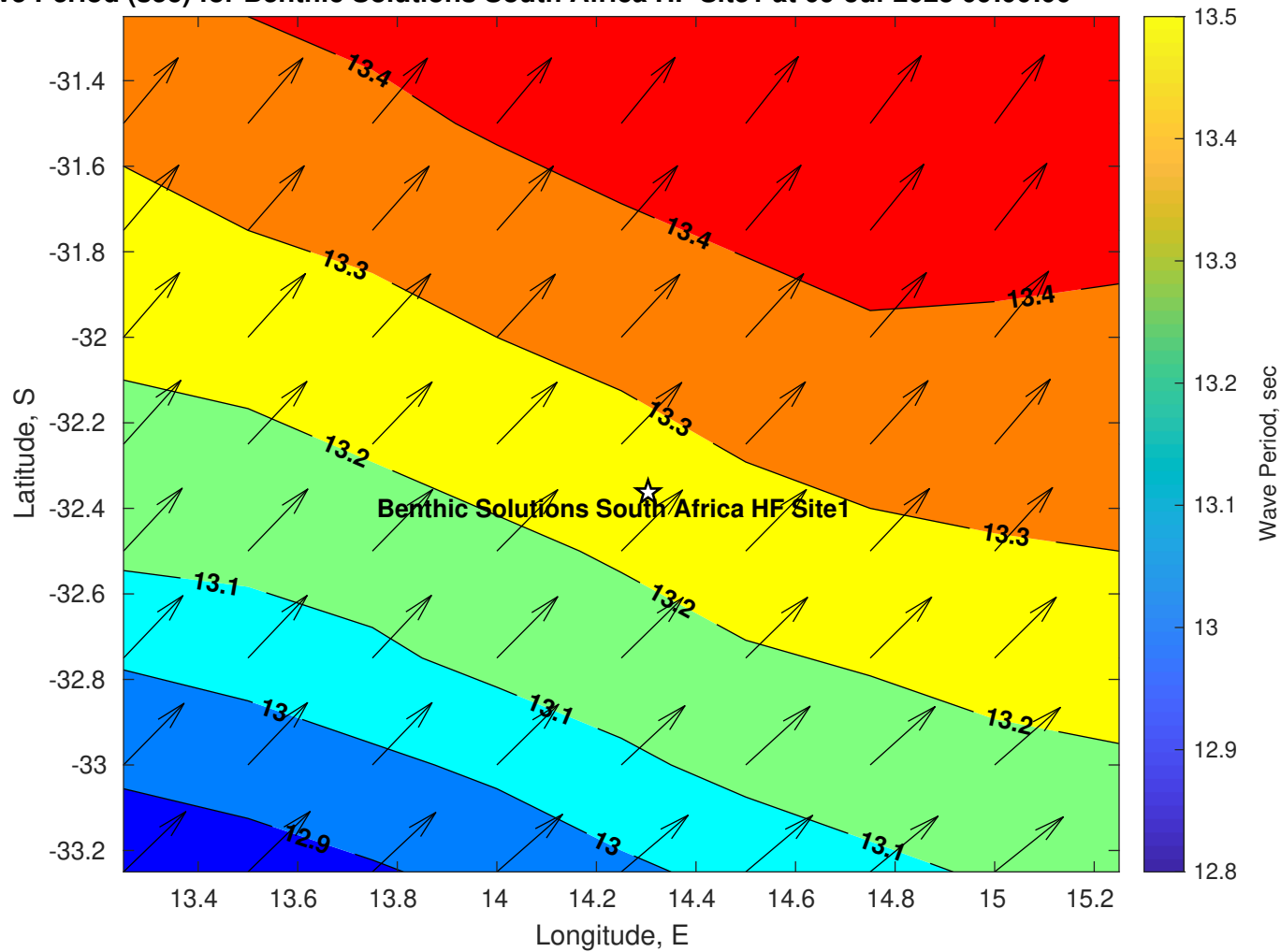
Wave Period (sec) for Benthic Solutions South Africa HF Site1 at 09-Jul-2025 09:00:00
