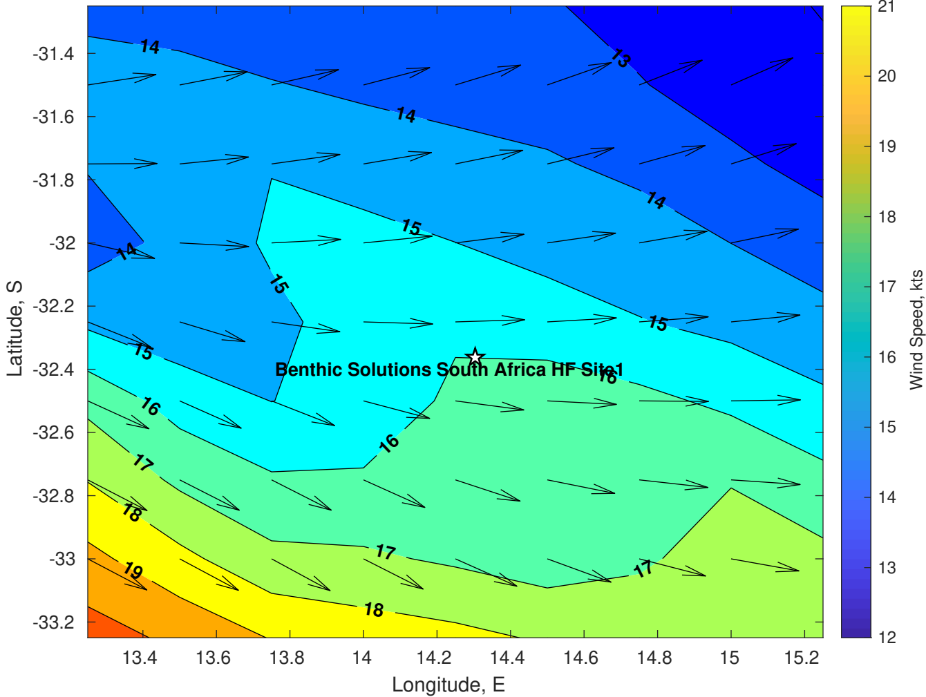
Winds (kts) for Benthic Solutions South Africa HF Site1 at 09-Jul-2025 09:00:00
