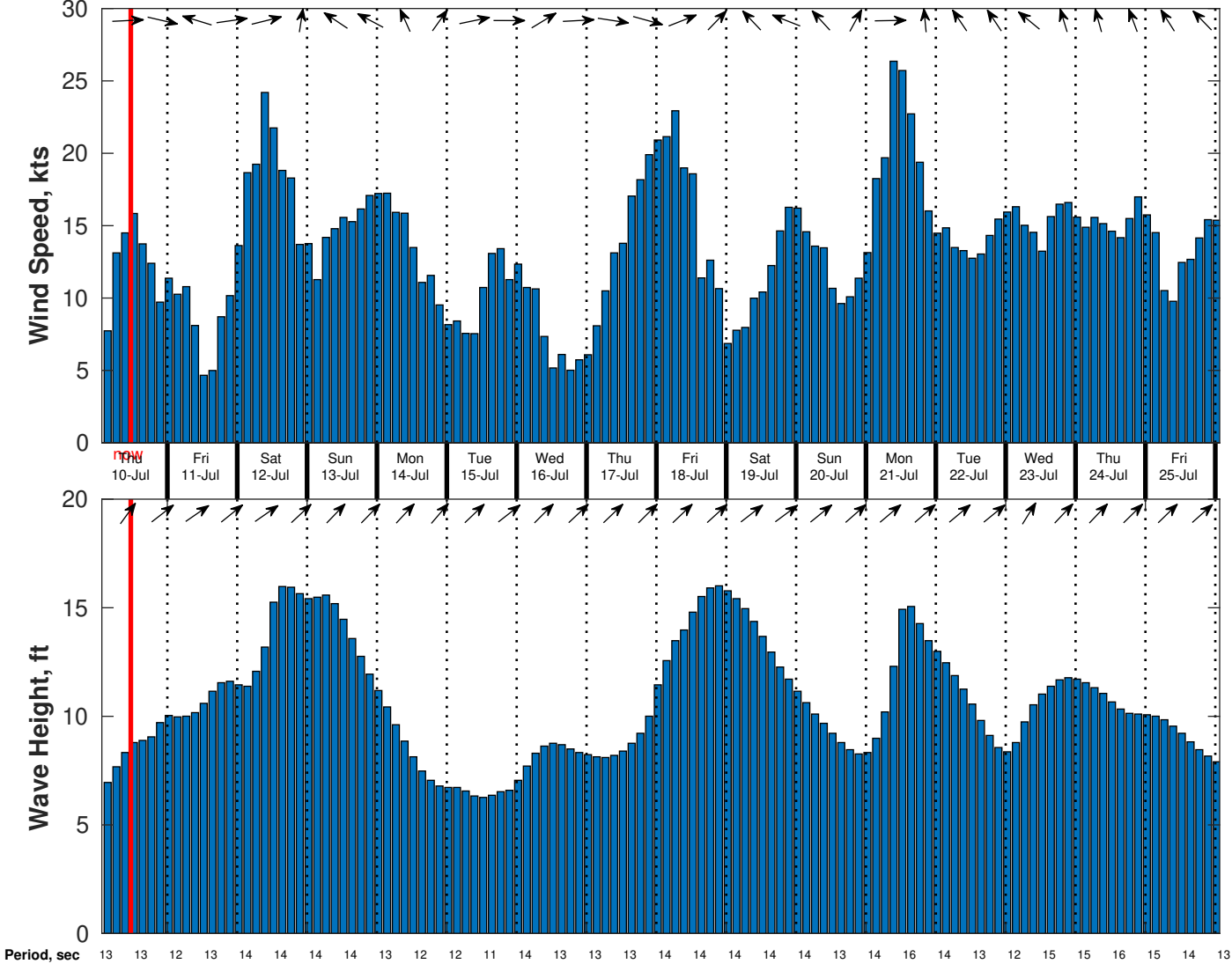
Wind & Wave Forecast for Benthic Solutions South Africa HF Site1 from 09-Jul-2025 02:00:00 to 25-Jul-2025 02:00:00
