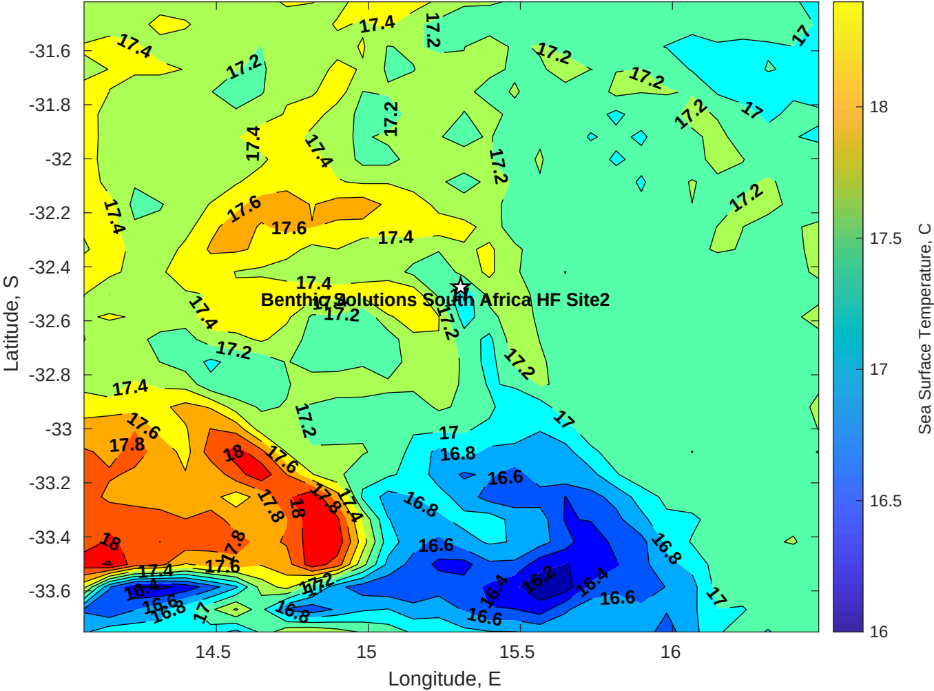
SST for Benthic Solutions South Africa HF Site2 at 08-Jul-2025 00:00:00
