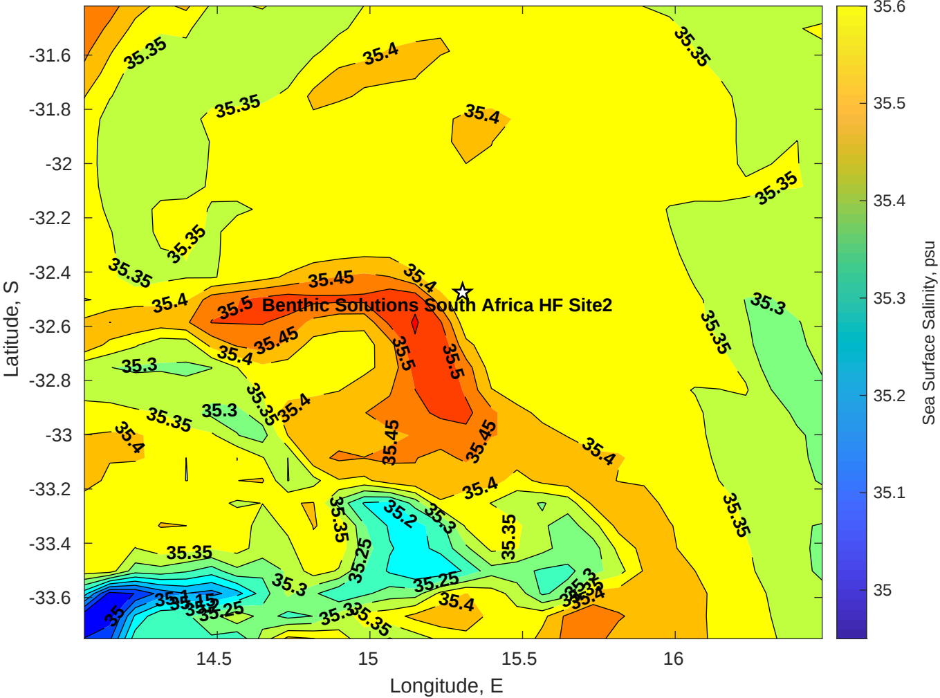
Surface Salinity for Benthic Solutions South Africa HF Site2 at 08-Jul-2025 00:00:00
