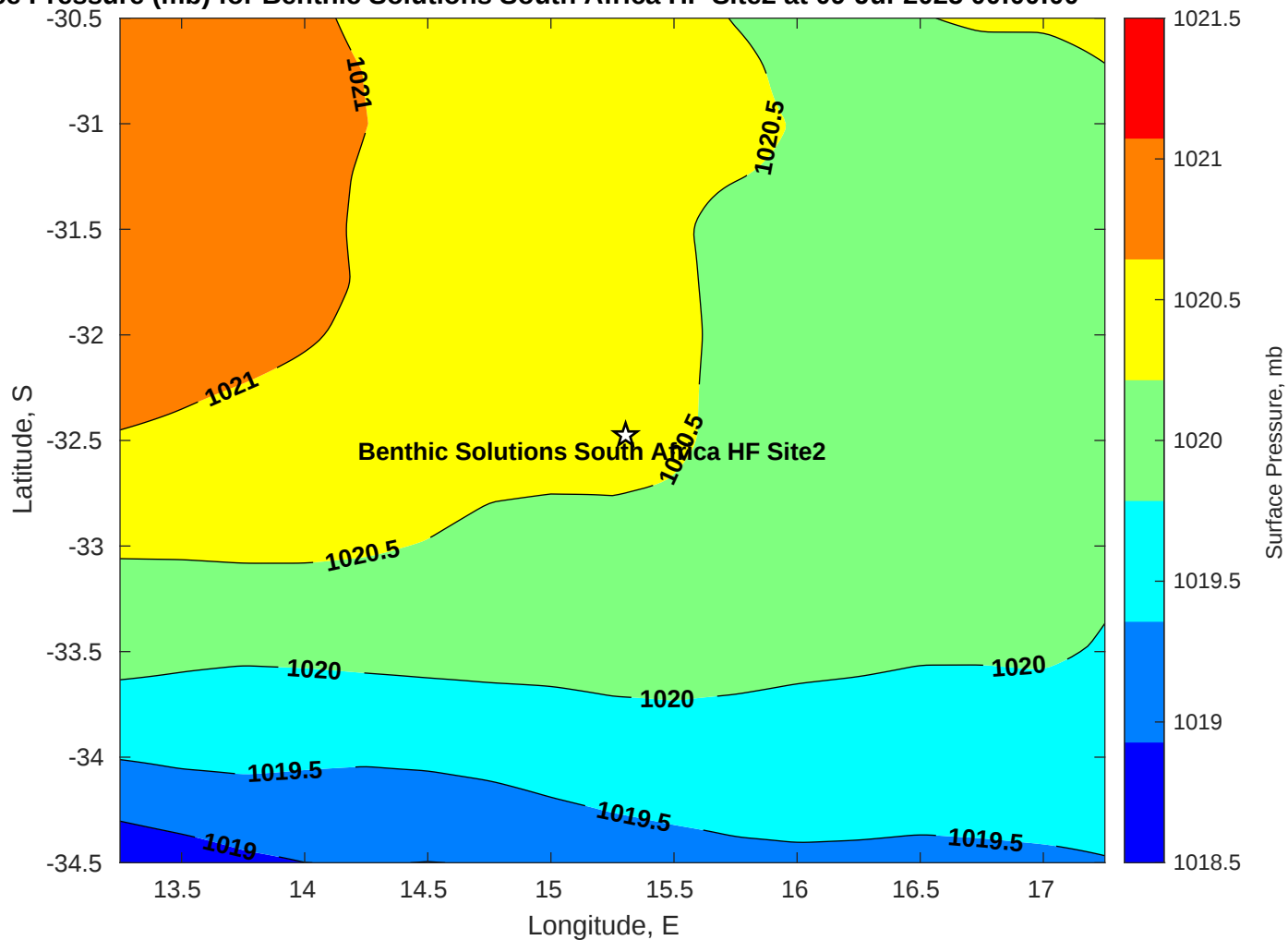
Surface Pressure (mb) for Benthic Solutions South Africa HF Site2 at 09-Jul-2025 00:00:00
