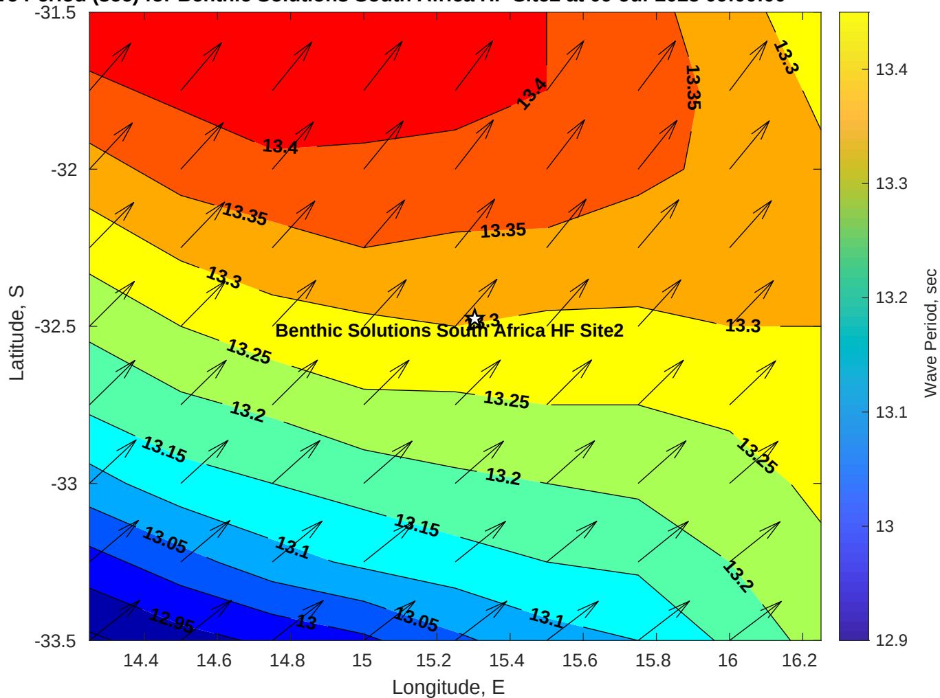
Wave Period (sec) for Benthic Solutions South Africa HF Site2 at 09-Jul-2025 09:00:00
