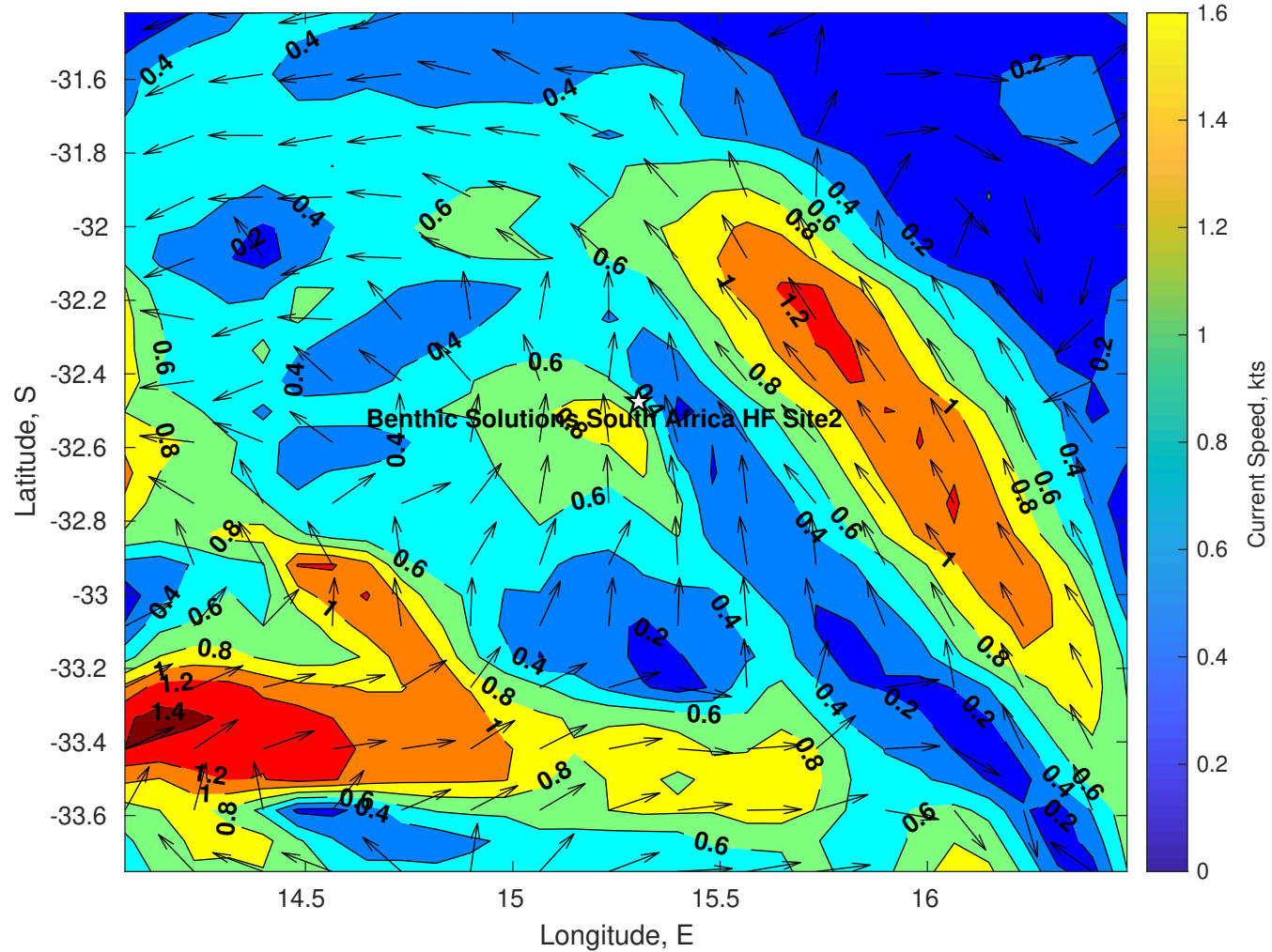
Surface Currents for Benthic Solutions South Africa HF Site2 at 08-Jul-2025 00:00:00
