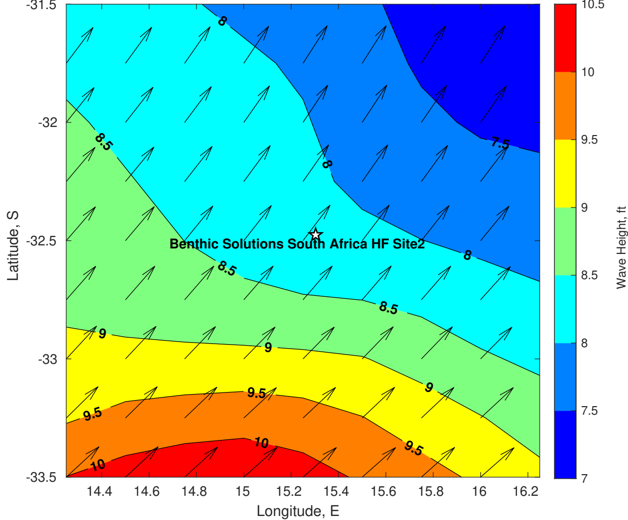
Wave Height (ft) for Benthic Solutions South Africa HF Site2 at 09-Jul-2025 09:00:00
