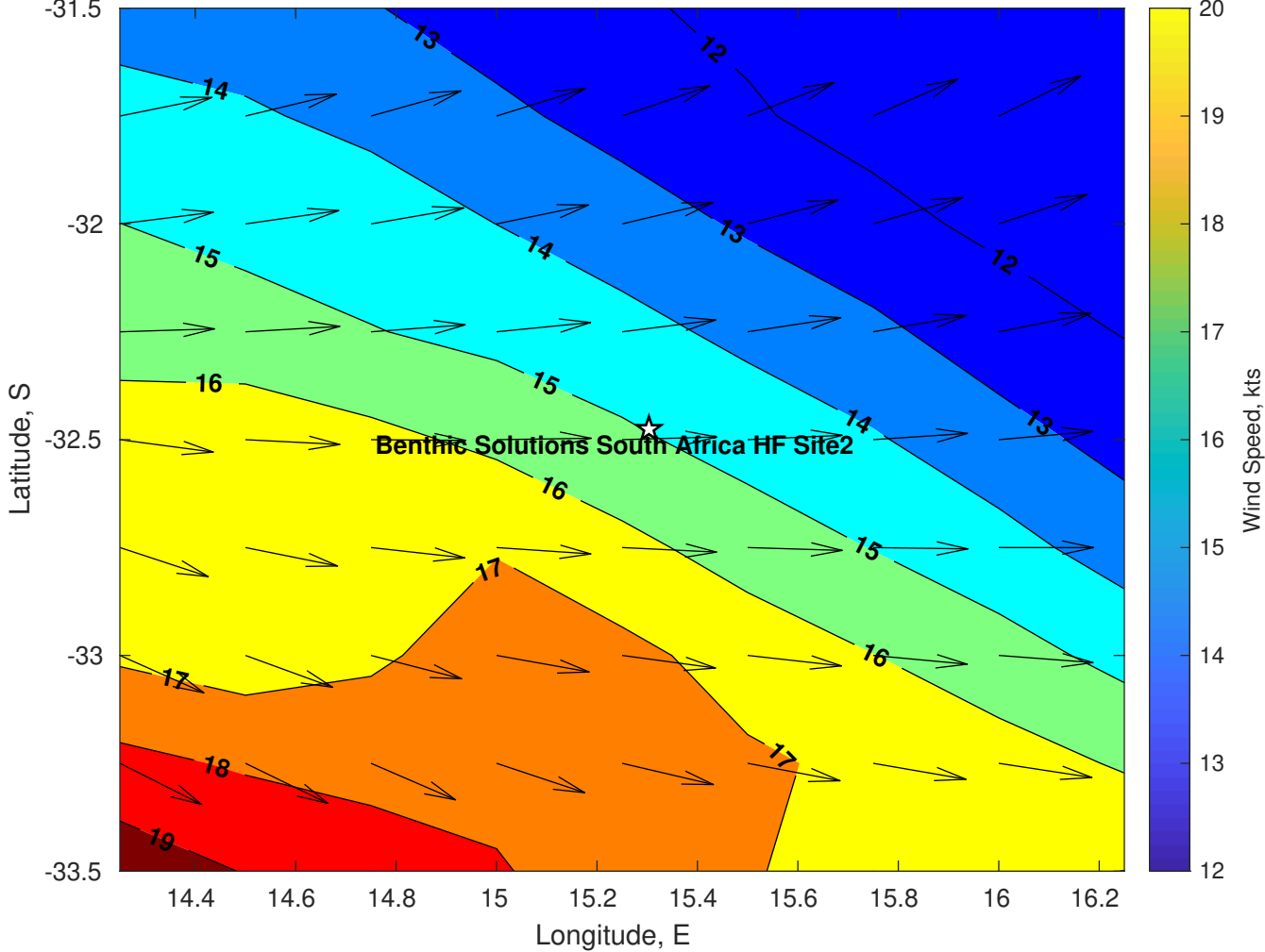
Winds (kts) for Benthic Solutions South Africa HF Site2 at 09-Jul-2025 09:00:00
