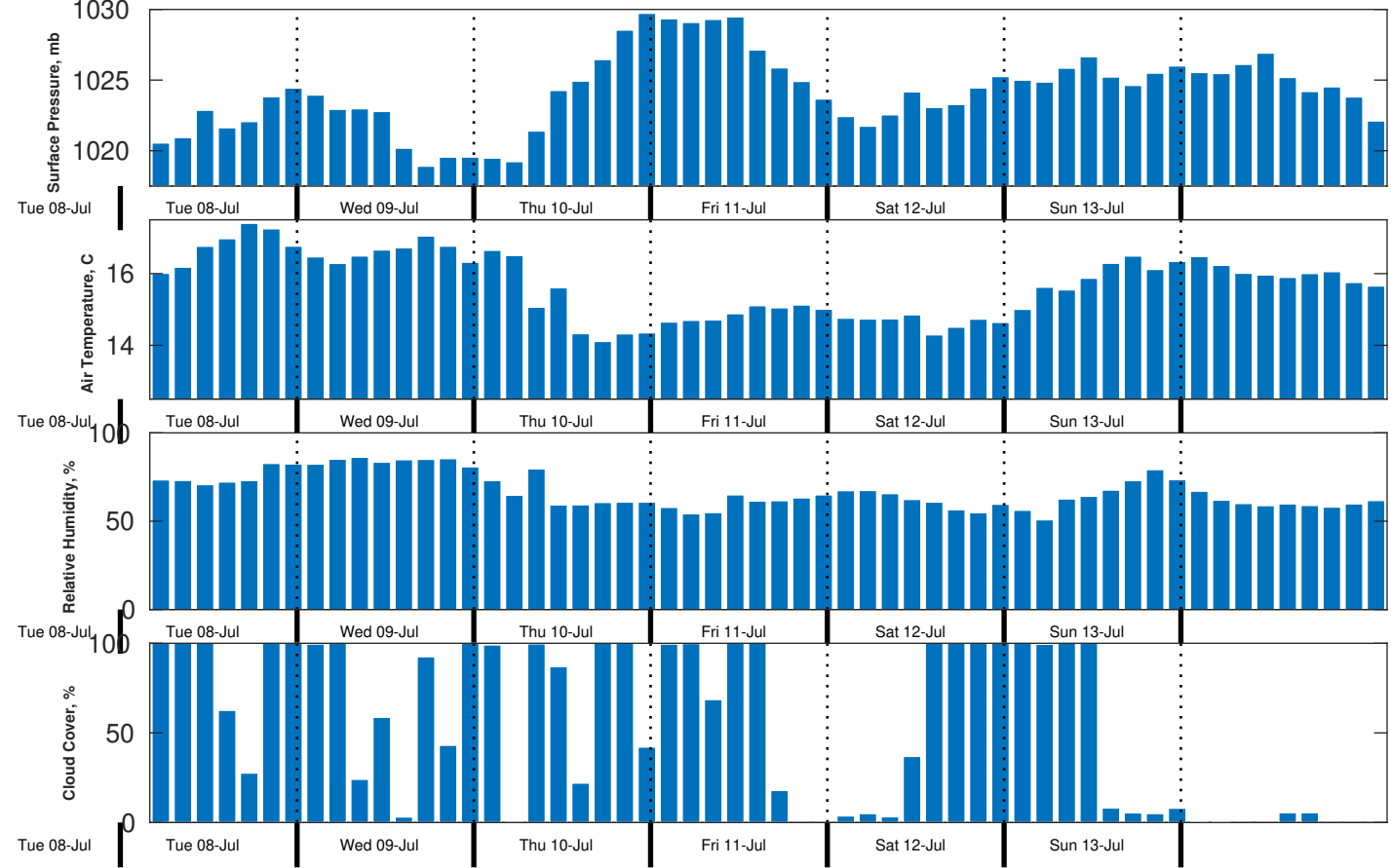
Met Forecast for Benthic Solutions South Africa HF Site2 from 09-Jul-2025 00:00:00 to 16-Jul-2025 00:00:00
