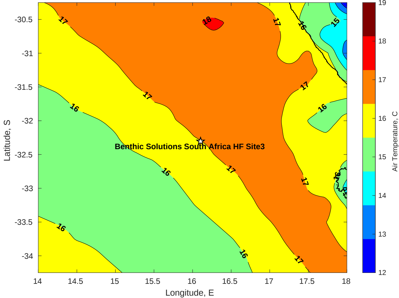
Air Temperature (C) for Benthic Solutions South Africa HF Site3 at 09-Jul-2025
