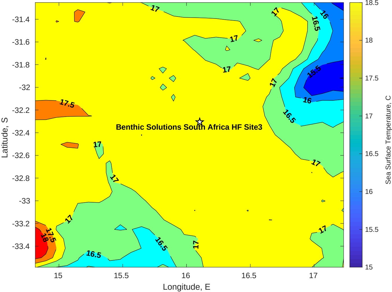
SST for Benthic Solutions South Africa HF Site3 at 08-Jul-2025 00:00:00
