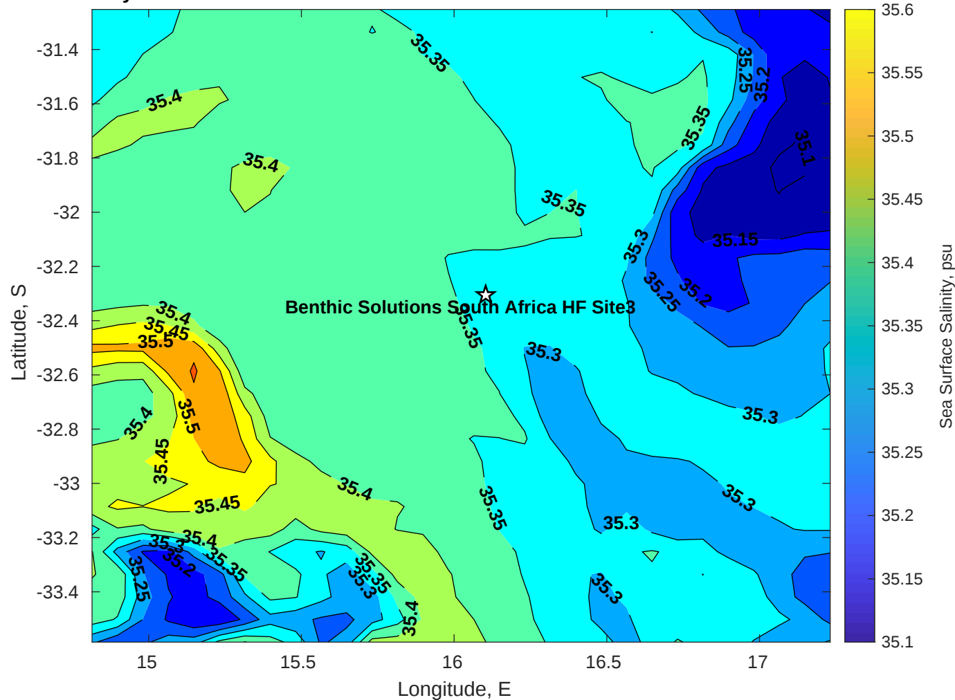
Surface Salinity for Benthic Solutions South Africa HF Site3 at 08-Jul-2025 00:00:00
