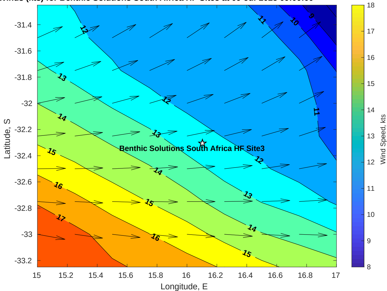
Winds (kts) for Benthic Solutions South Africa HF Site3 at 09-Jul-2025 09:00:00
