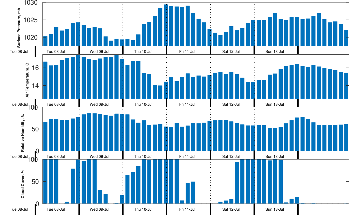
Met Forecast for Benthic Solutions South Africa HF Site3 from 09-Jul-2025 00:00:00 to 16-Jul-2025 00:00:00
