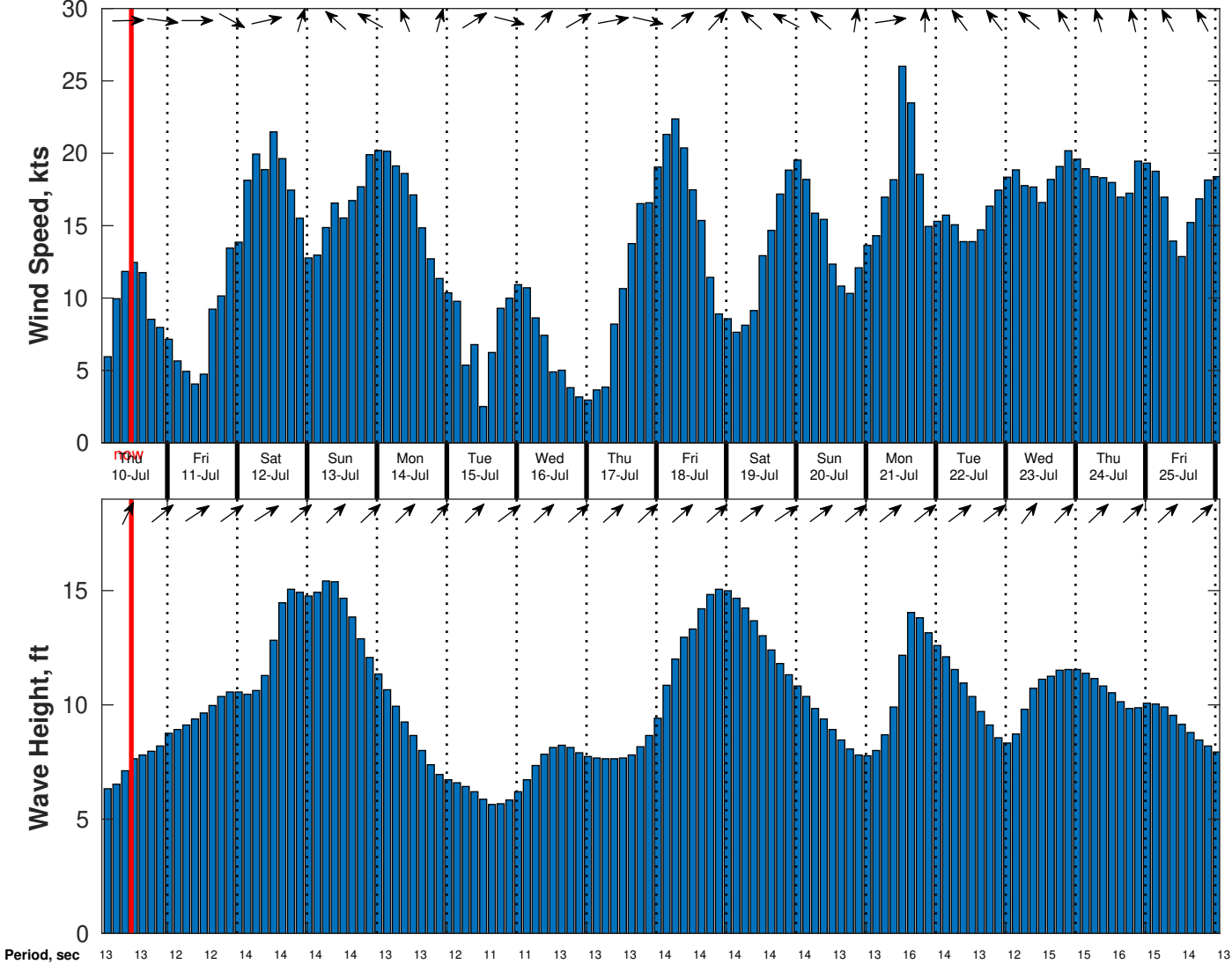
Wind & Wave Forecast for Benthic Solutions South Africa HF Site3 from 09-Jul-2025 02:00:00 to 25-Jul-2025 02:00:00
