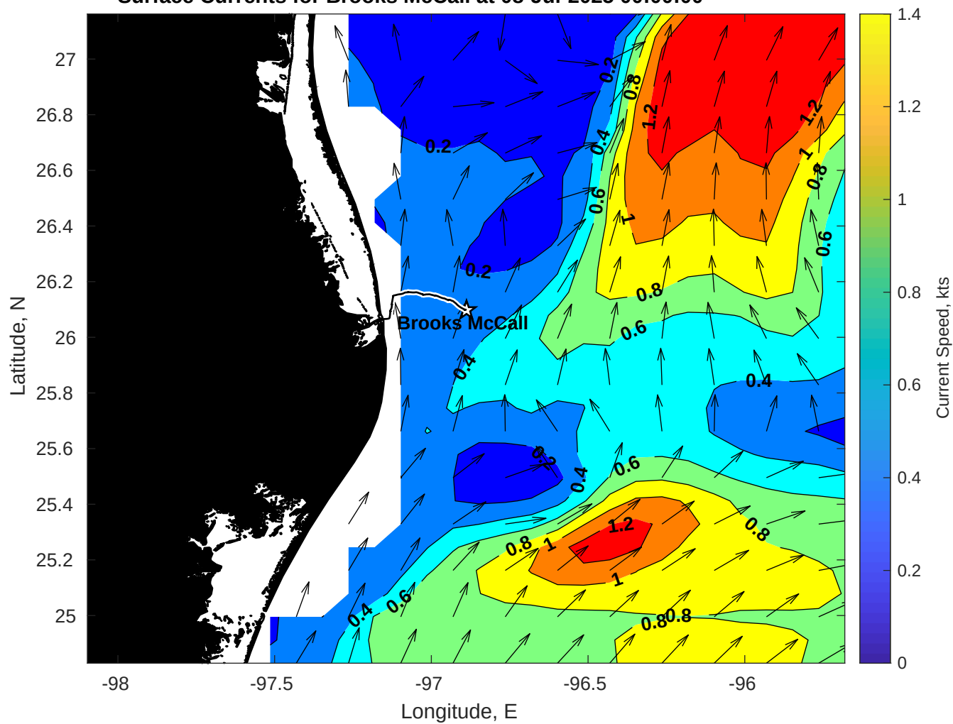
Surface Currents for Brooks McCall at 08-Jul-2025 00:00:00
