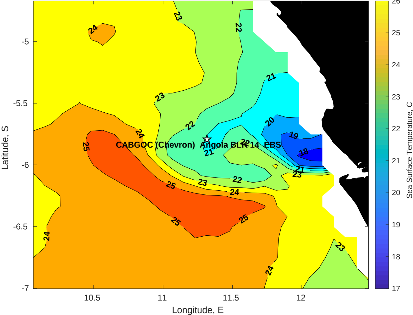
SST for CABGOC (Chevron) Angola BLK 14 EBS at 08-Jul-2025 00:00:00
