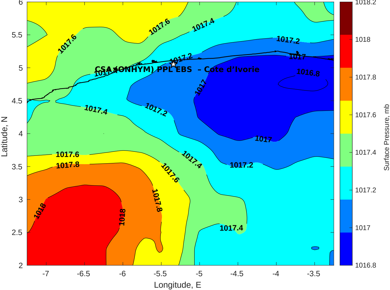
Surface Pressure (mb) for CSA (ONHYM) PPL EBS - Cote d'Ivoire at 09-Jul-2025 00:00:00
