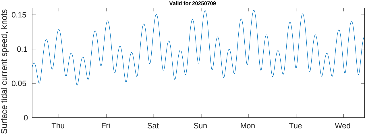
Tidal Currents and Heights for CSA (ONHYM) PPL EBS - Cote d'Ivoire at 20250709
