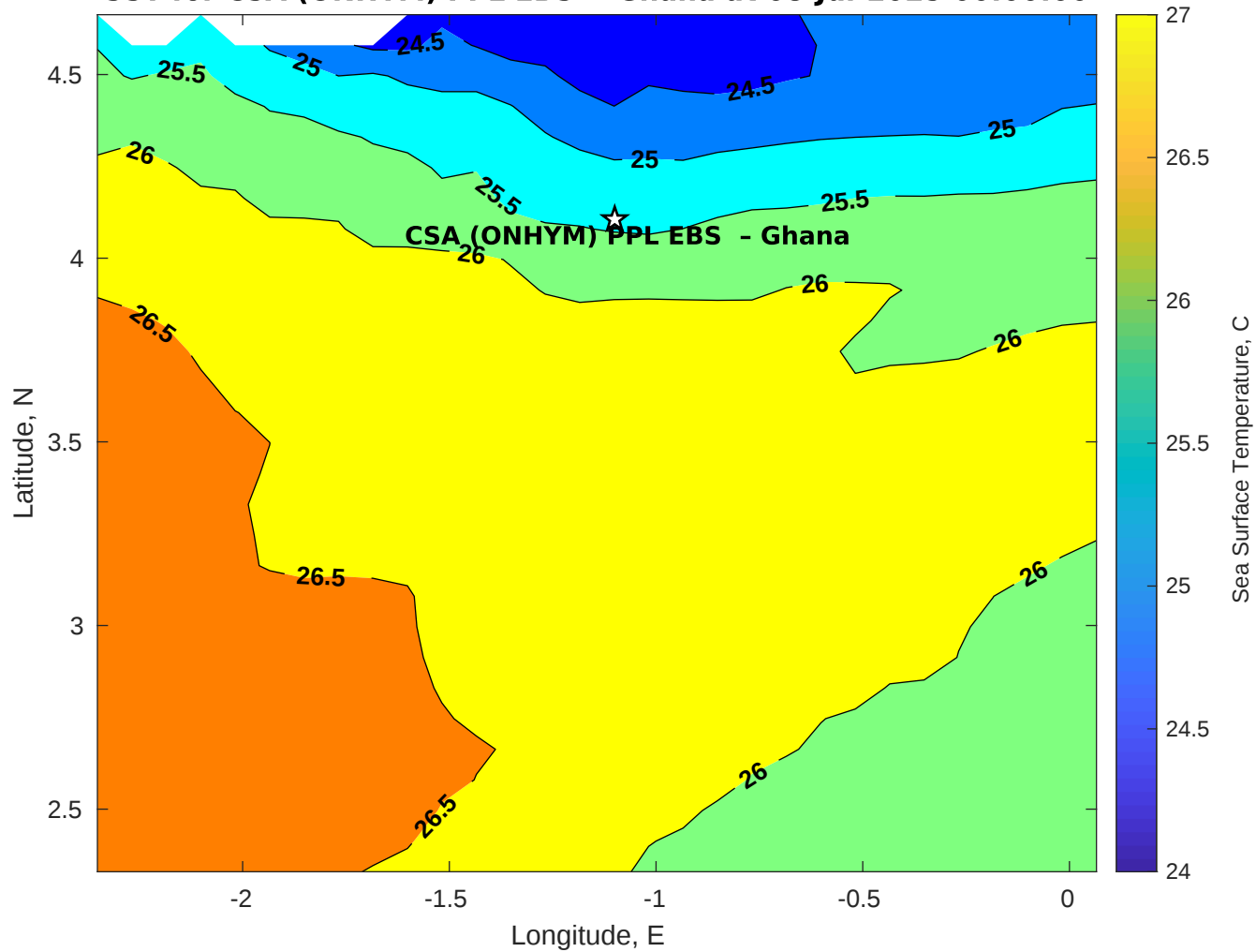
SST for CSA (ONHYM) PPL EBS - Ghana at 08-Jul-2025 00:00:00
