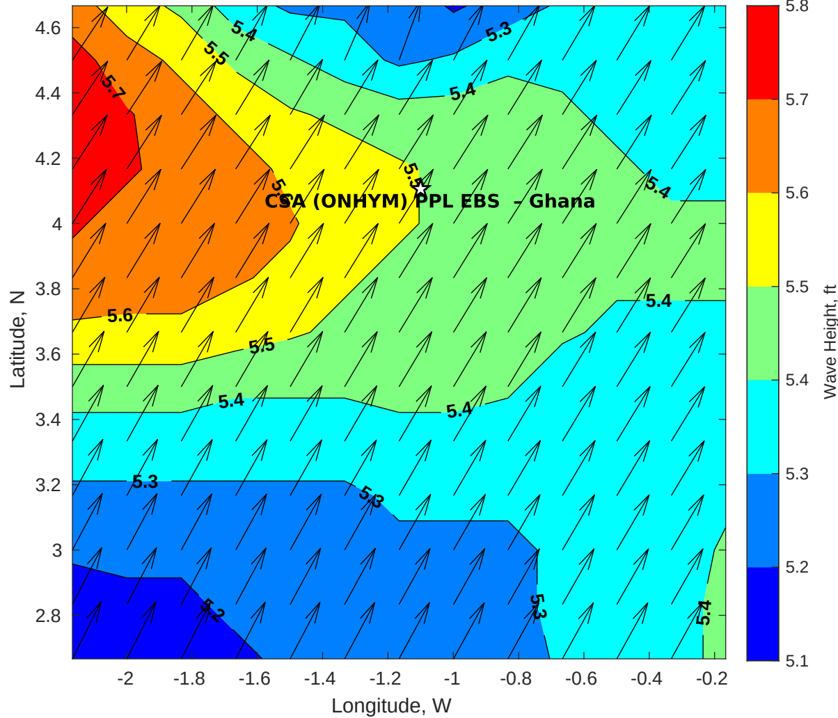
Wave Height (ft) for CSA (ONHYM) PPL EBS - Ghana at 09-Jul-2025 09:00:00
