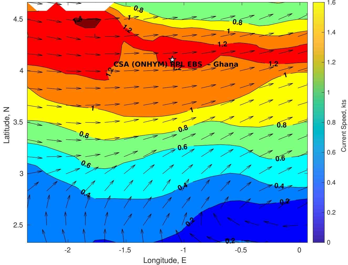
Surface Currents for CSA (ONHYM) PPL EBS - Ghana at 08-Jul-2025 00:00:00
