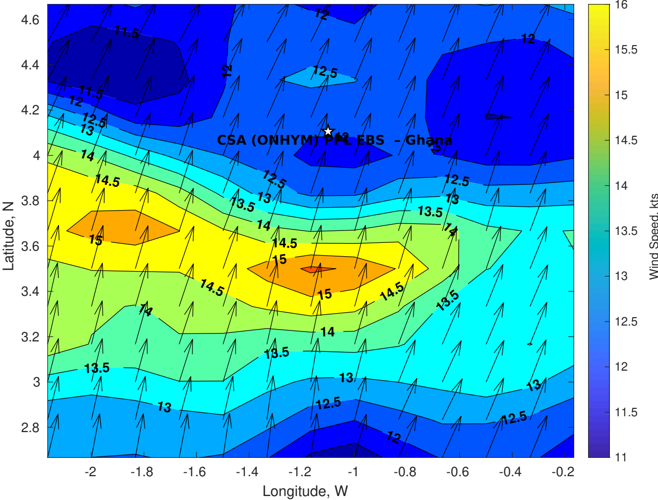
Winds (kts) for CSA (ONHYM) PPL EBS - Ghana at 09-Jul-2025 09:00:00
