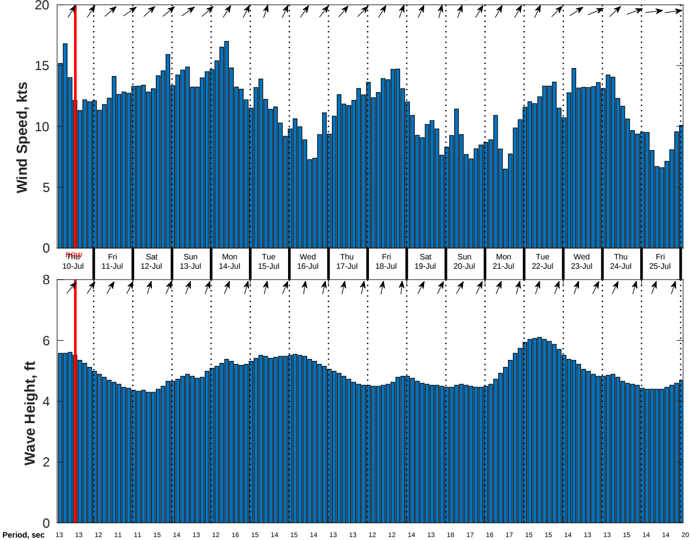
Wind & Wave Forecast for CSA (ONHYM) PPL EBS - Ghana from 09-Jul-2025 02:00:00 to 25-Jul-2025 02:00:00
