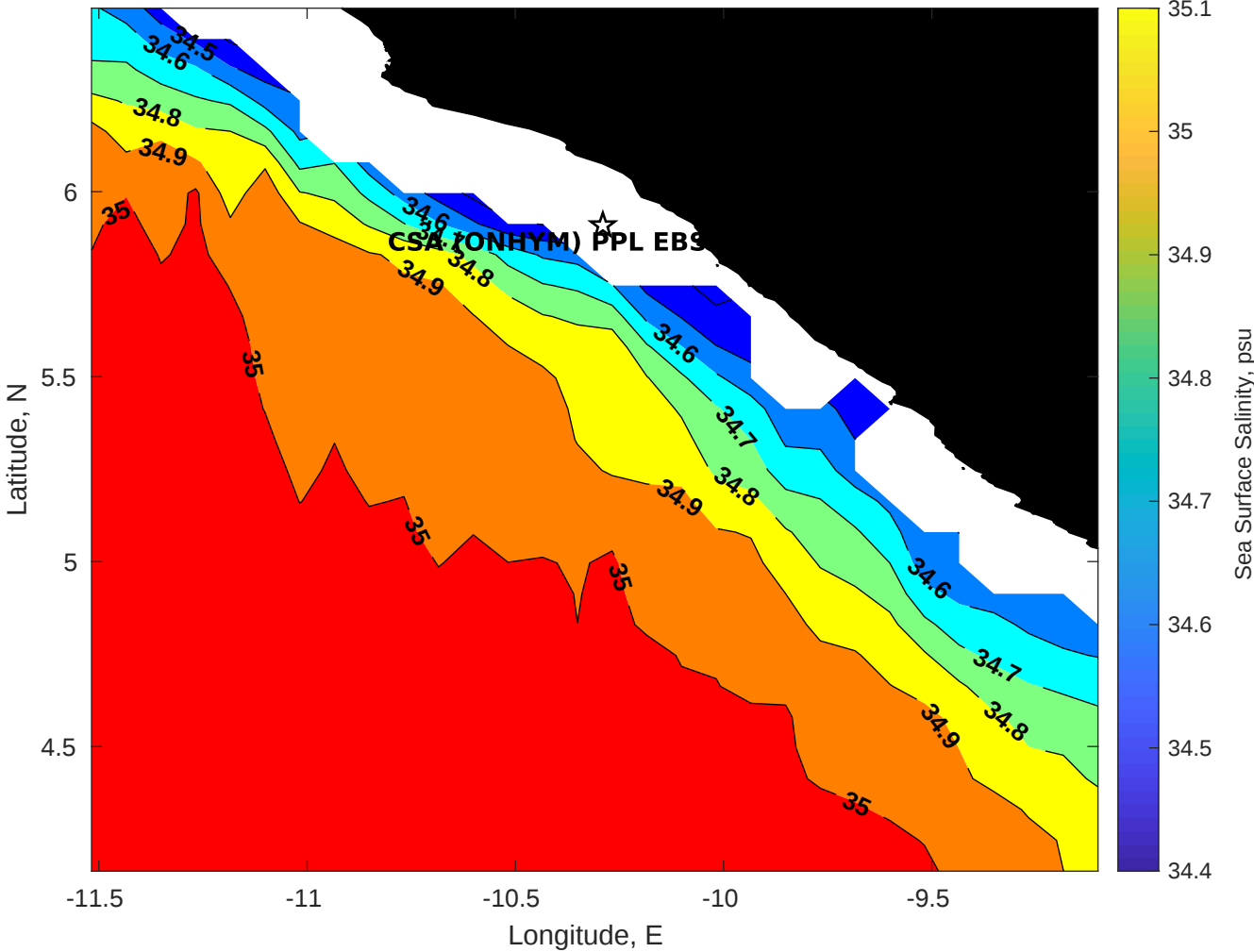
Surface Salinity for CSA (ONHYM) PPL EBS - Liberia at 08-Jul-2025 00:00:00
