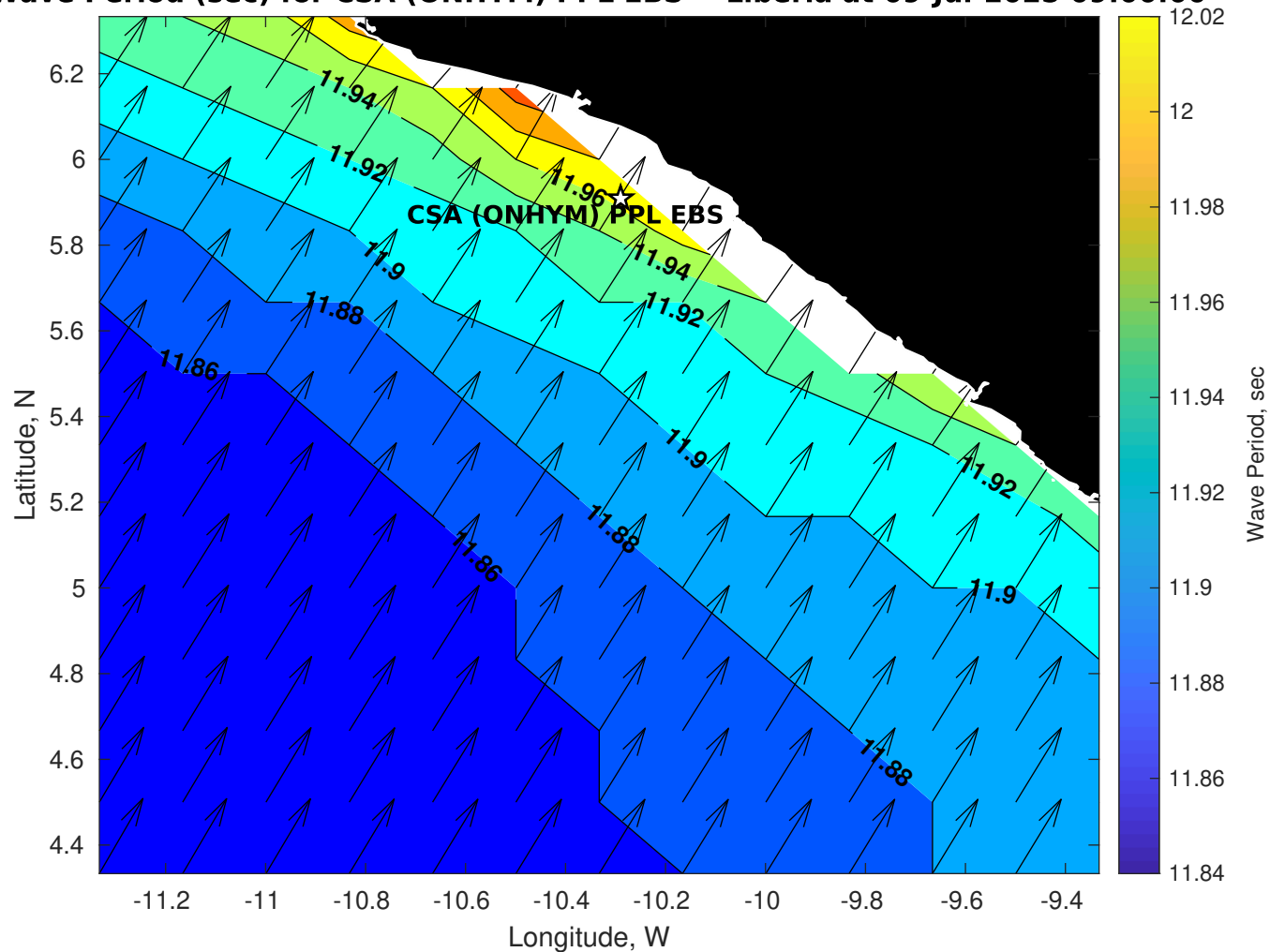
Wave Period (sec) for CSA (ONHYM) PPL EBS - Liberia at 09-Jul-2025 09:00:00
