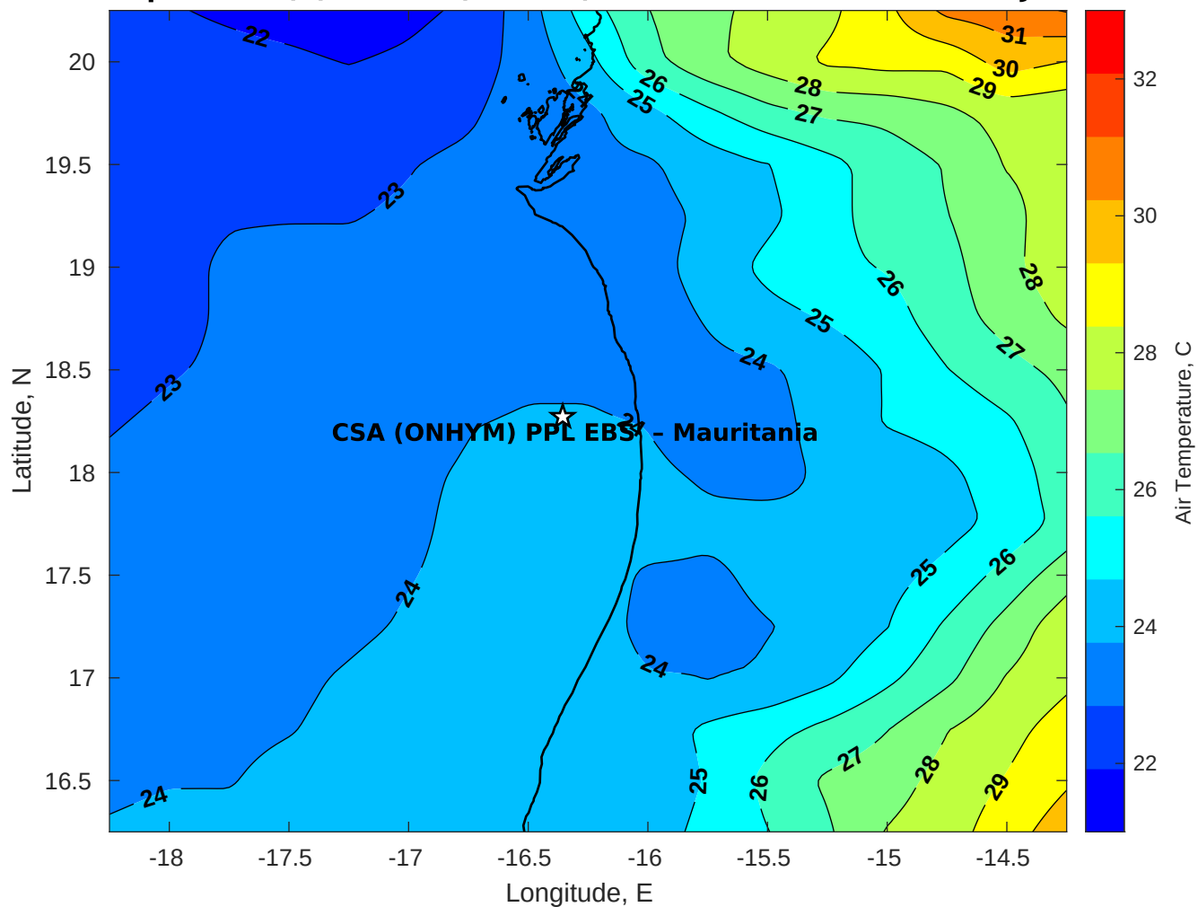
Air Temperature (C) for CSA (ONHYM) PPL EBS - Mauritania at 09-Jul-2025
