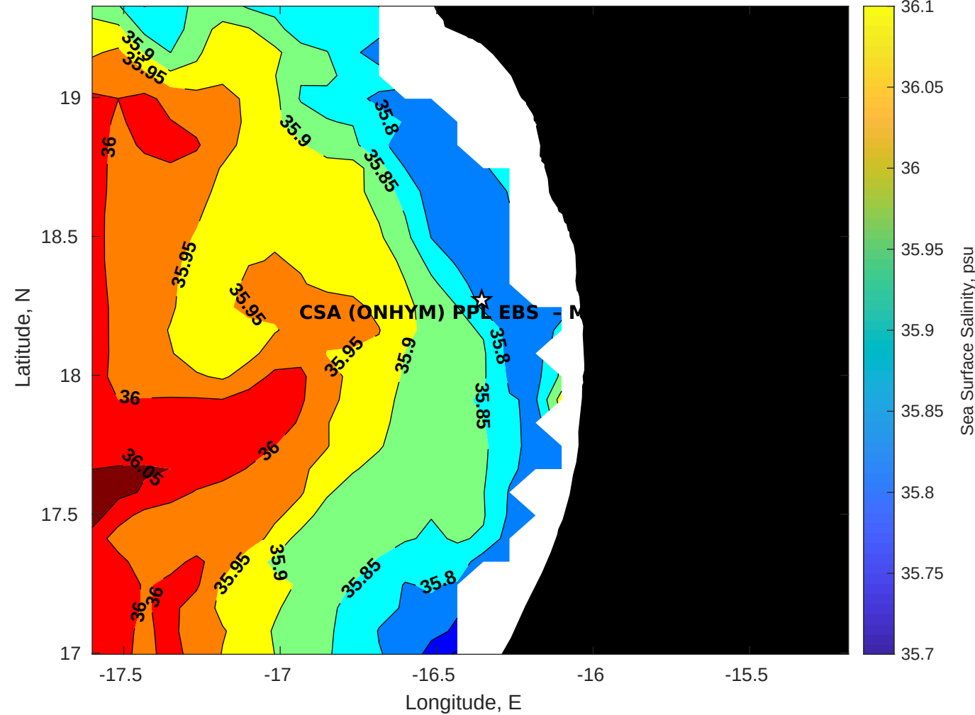
Surface Salinity for CSA (ONHYM) PPL EBS - Mauritania at 08-Jul-2025 00:00:00
