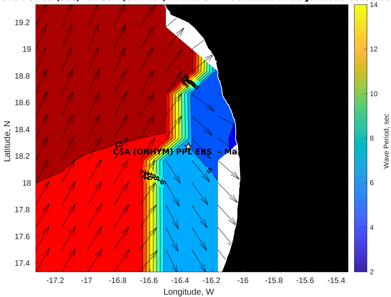
Wave Period (sec) for CSA (ONHYM) PPL EBS - Mauritania at 09-Jul-2025 09:00:00
