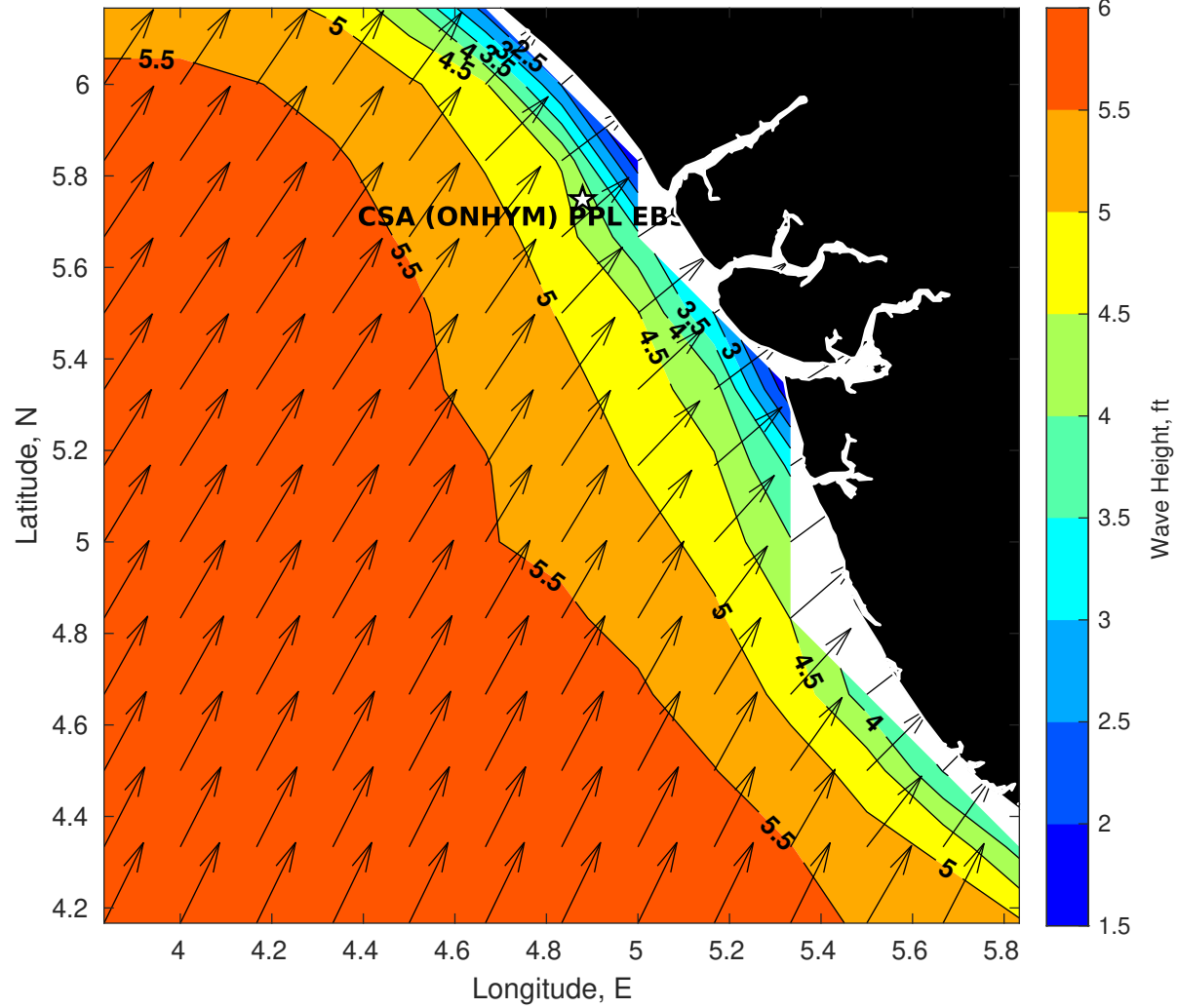
Wave Height (ft) for CSA (ONHYM) PPL EBS - Nigeria at 09-Jul-2025 09:00:00
